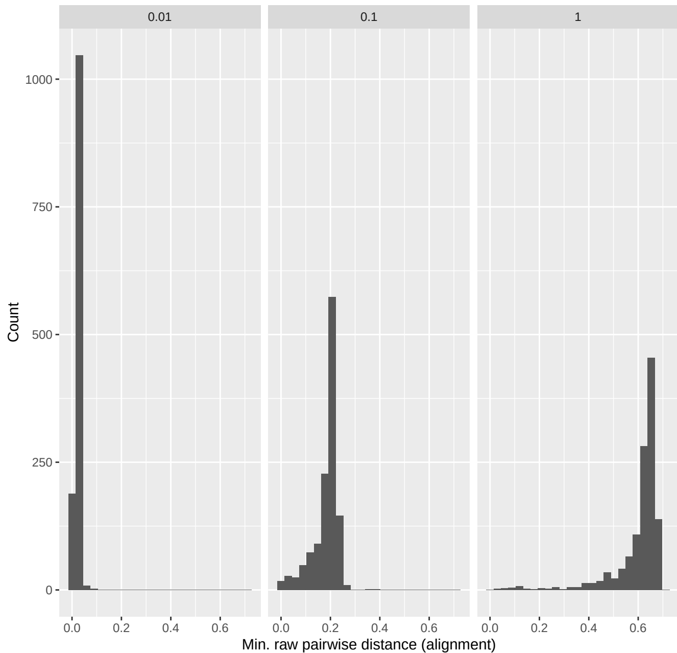
B2: Alignment pairwise distances (model = raw) for three tree depths
