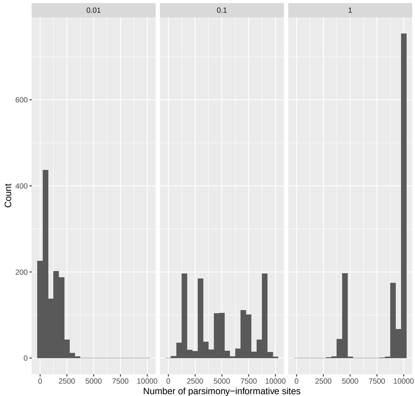
B2: Parsimony-informative sites for three tree depths
