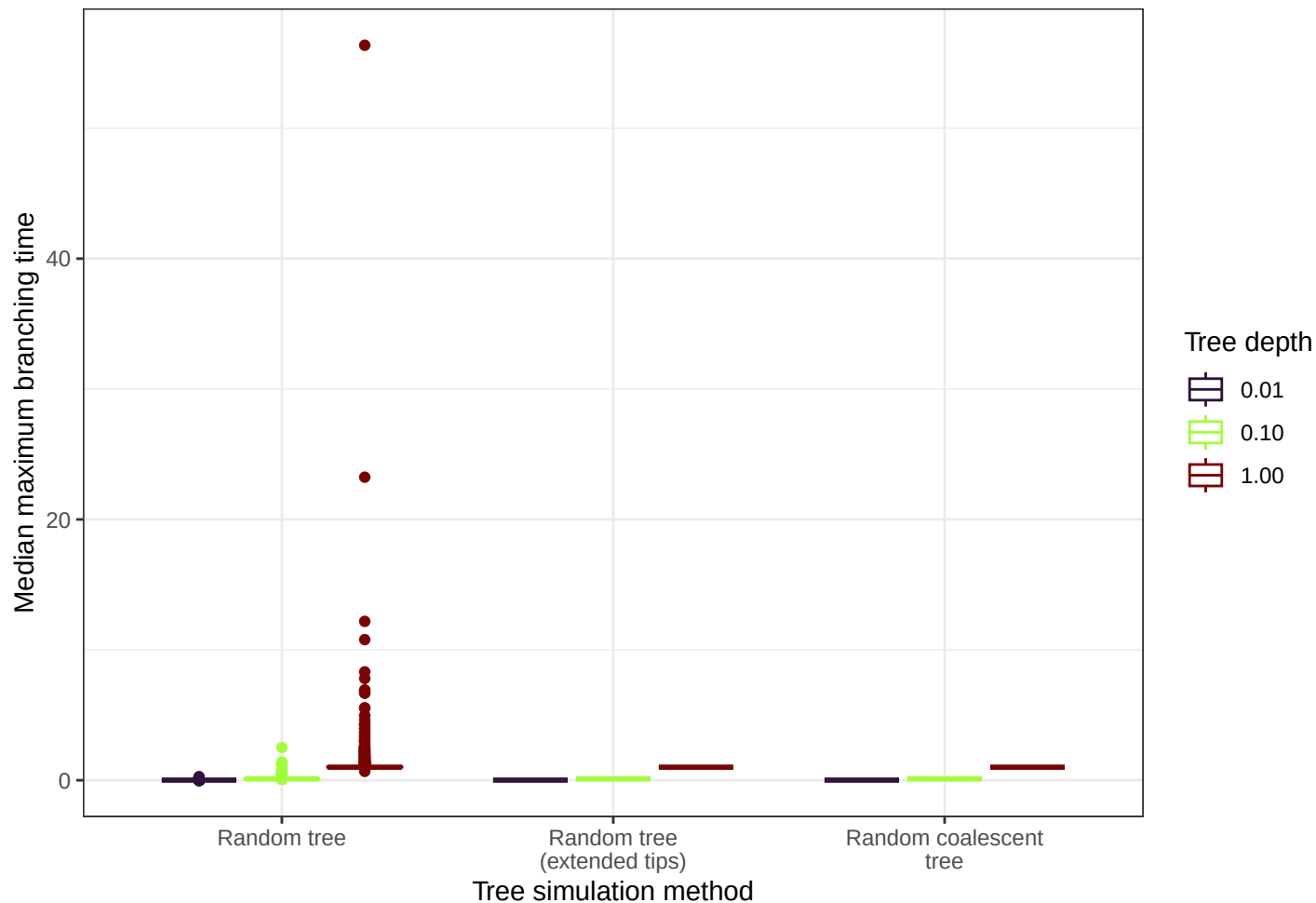
Median maximum branching time for all random trees generated by three methods
