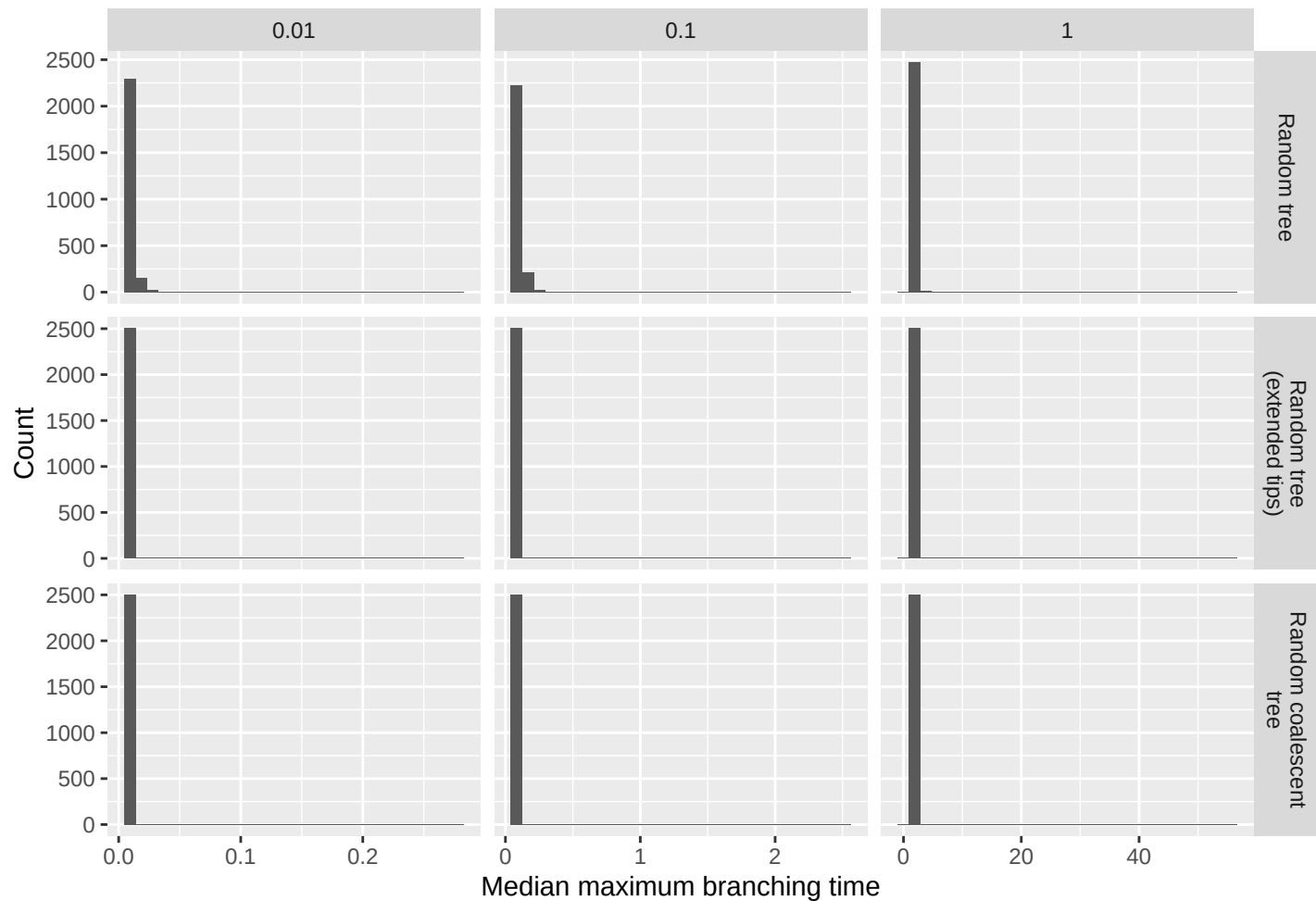
Median maximum branching time for all random trees in a single simulation replicate
