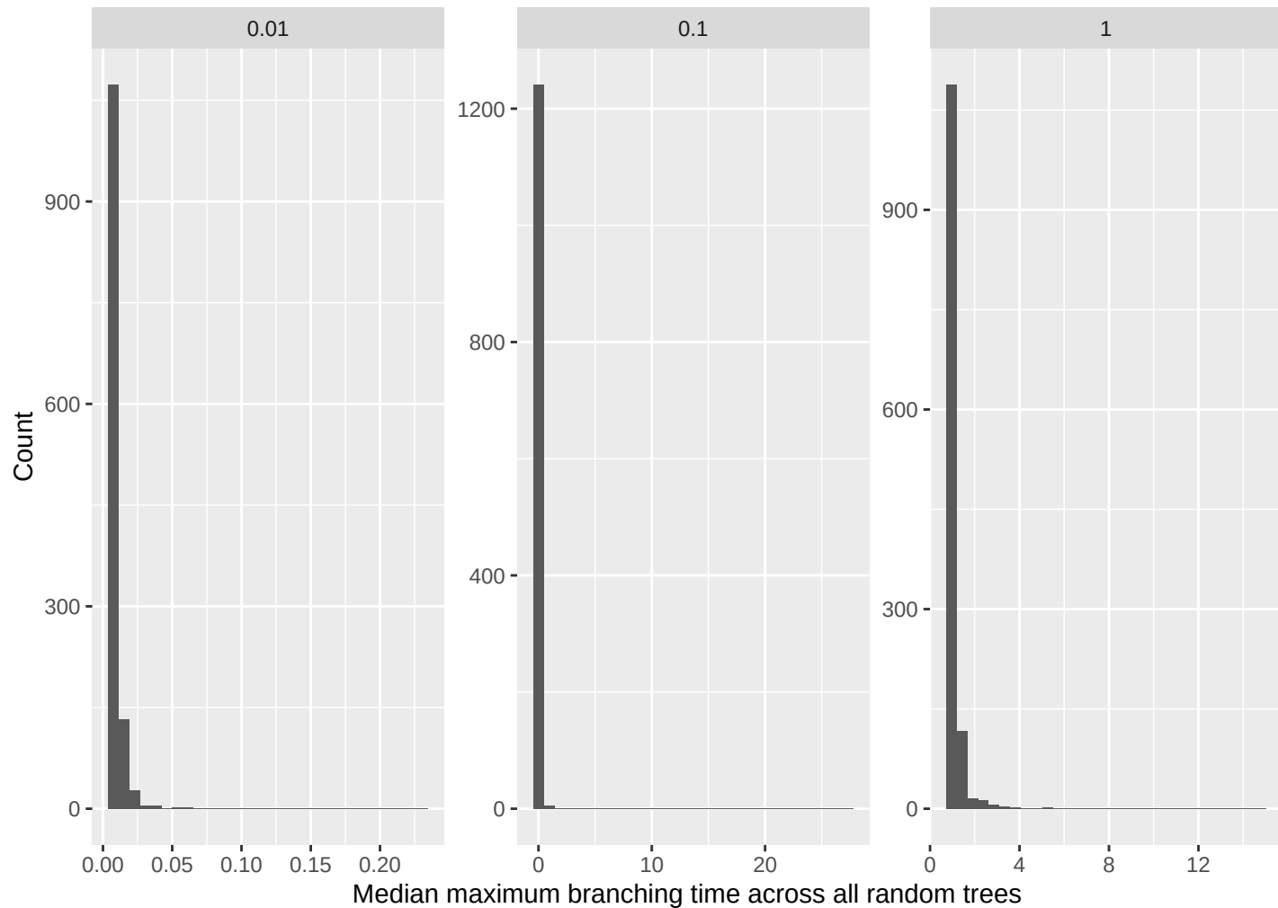
B2: Randomly generated trees – maximum branching time for three tree depths
