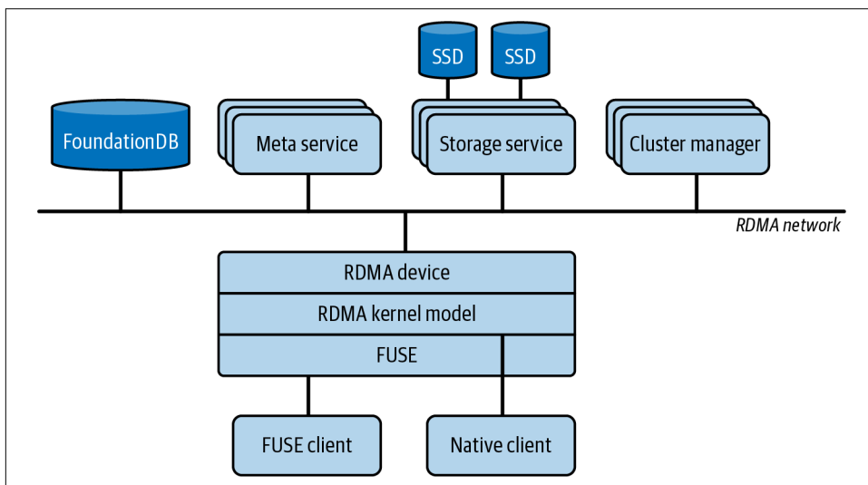
Figure 5-2. Components of DeepSeek's Fire-Flyer File System (3FS) (source: https://oreil.ly/xD3id )
