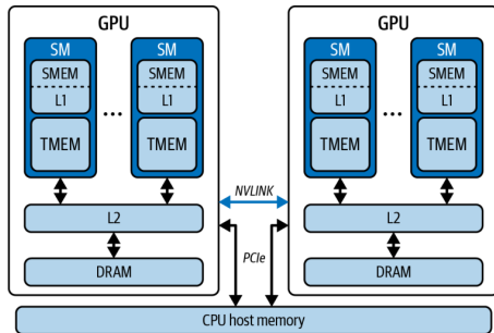
Figure 6-10. GPU memory hierarchy, including the CPU
