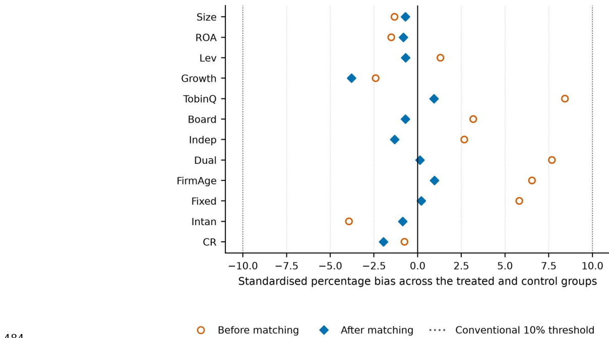
485 Figure 3. Covariate balance before and after propensity-score matching.
