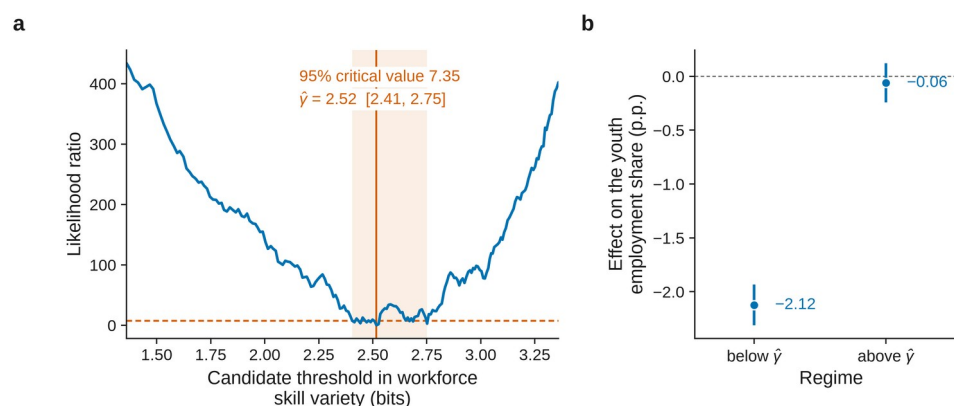
Figure 3. The requisite-variety threshold and the regime-specific shock coefficients.
