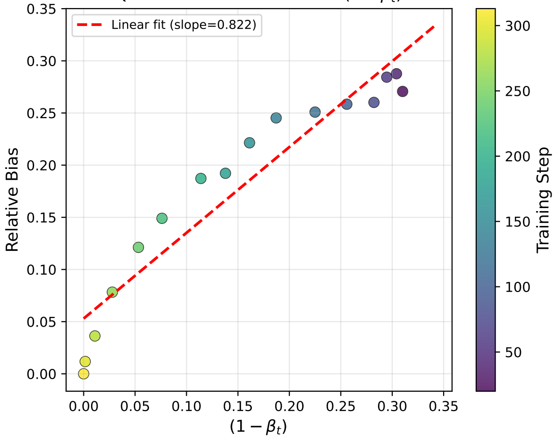
Qwen2.5-Math-1.5B: Bias \propto (1 - \beta_t)
