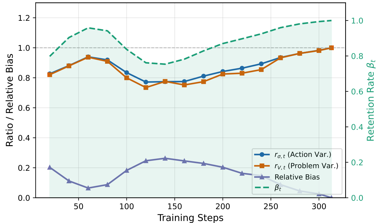
Qwen2.5-Math-1.5B (Oracle)
