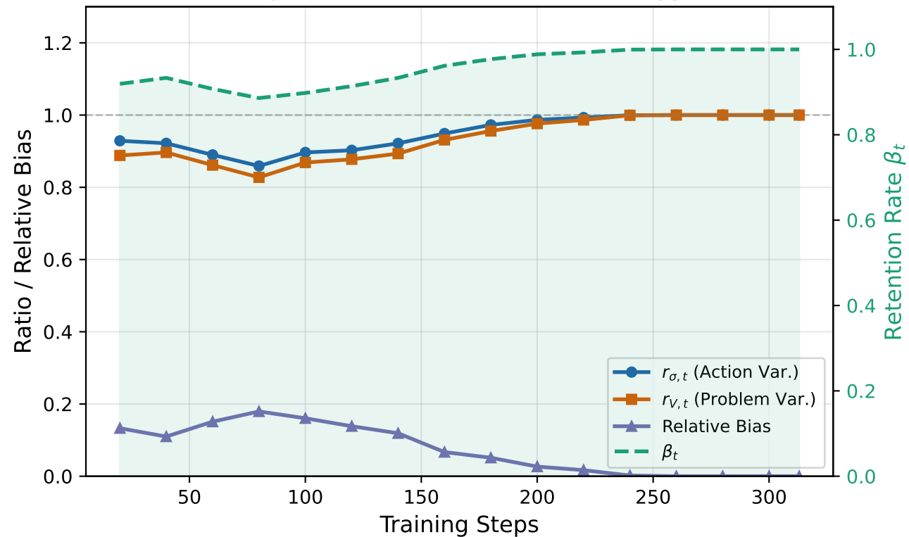
DeepSeek-R1-Distill-Qwen-1.5B (Entropy)
