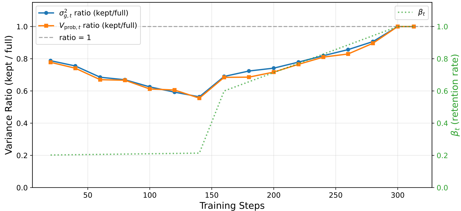
Qwen2.5-Math-1.5B (Oracle, VI-CuRL) - Variance Reduction
