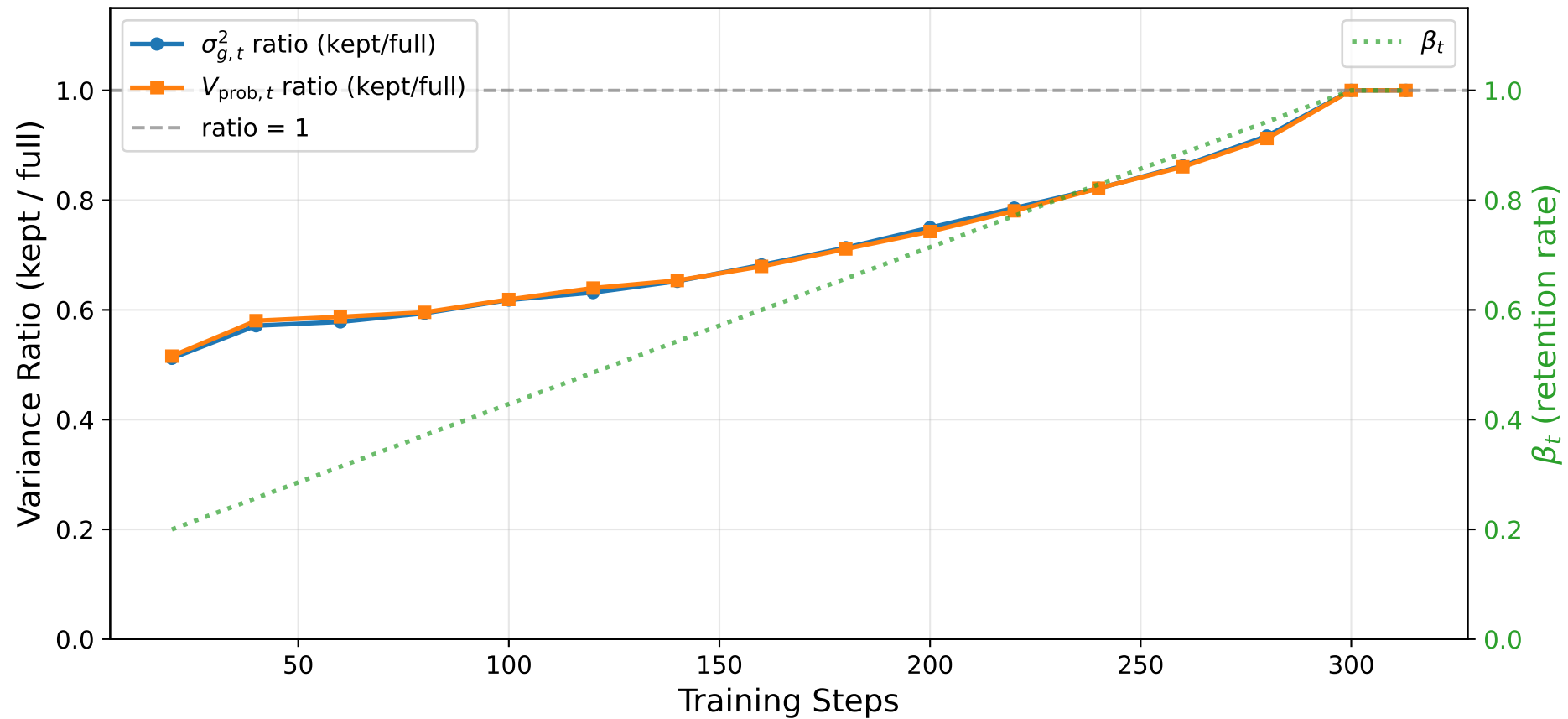
Qwen2.5-Math-1.5B (Oracle, No-CuRL) - Variance Reduction
