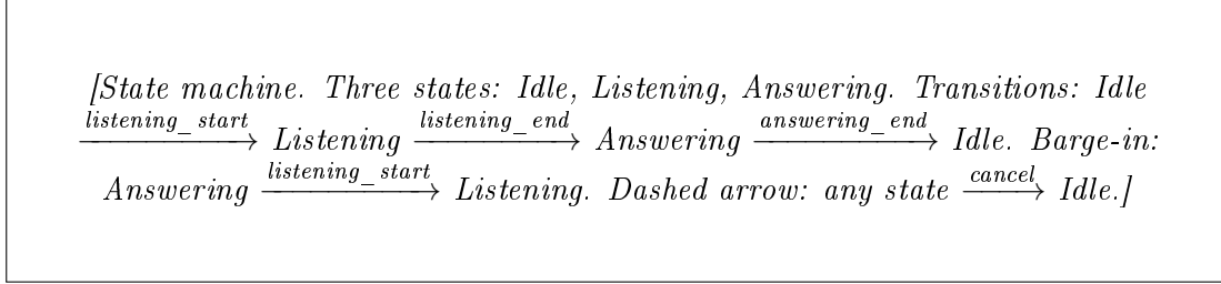
Figure 5: Client-side state machine governing agent behavior.
