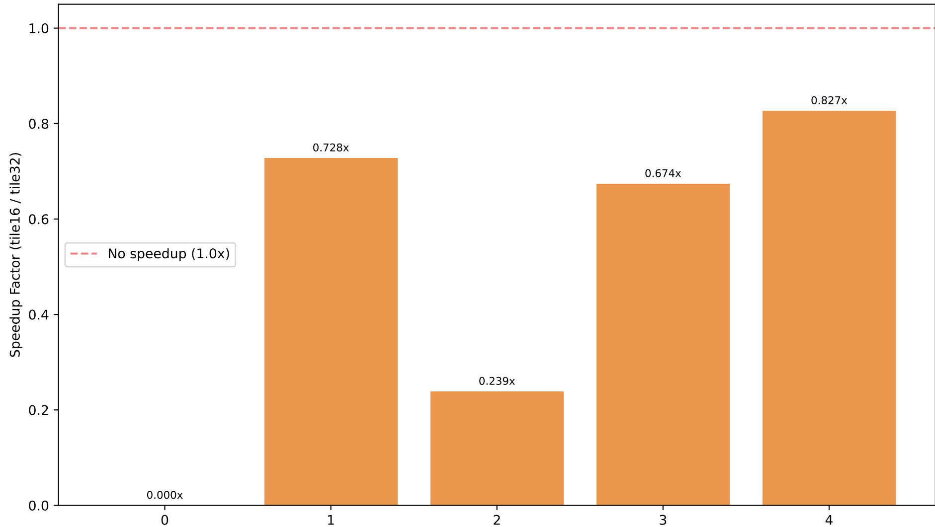
tile32 Speedup: Official Scenes vs Synthetic Workloads
