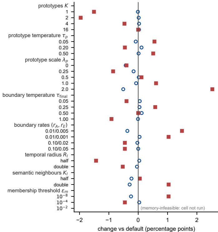
(a) hyper-parameter sensitivity
