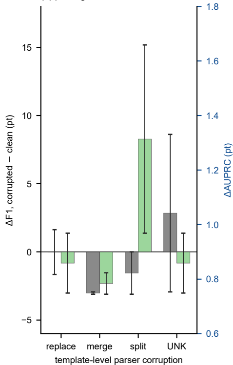
(b) parsing-noise robustness
