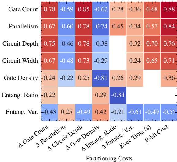
Input Circuit Properties
