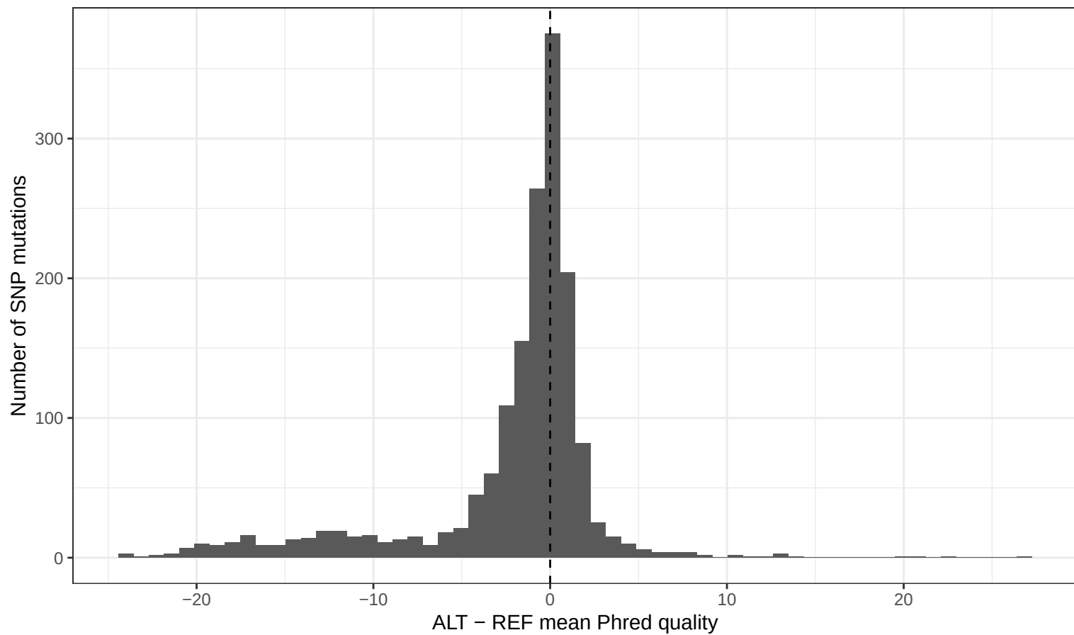
ALT-supporting bases show a modest Phred reduction
