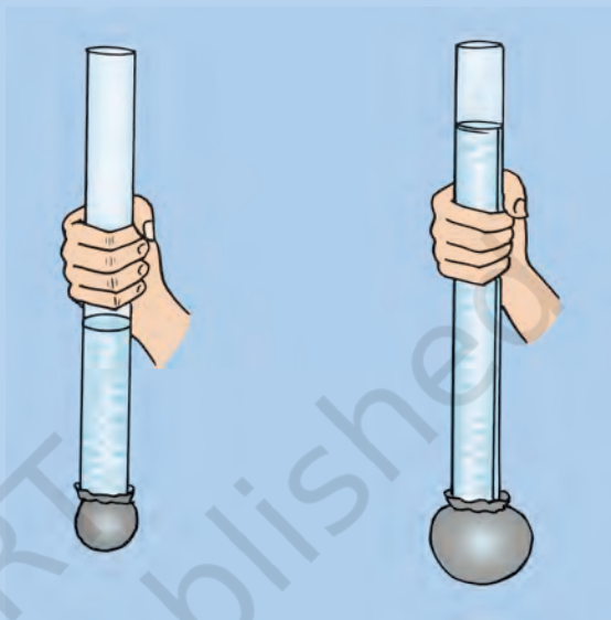
Fig. 8.14 : Pressure exerted by water at the bottom of the container depends on the height of its column
