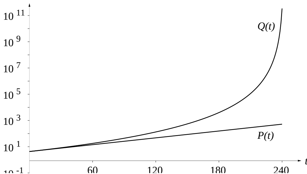
The graphs of P(t) and Q(t)
