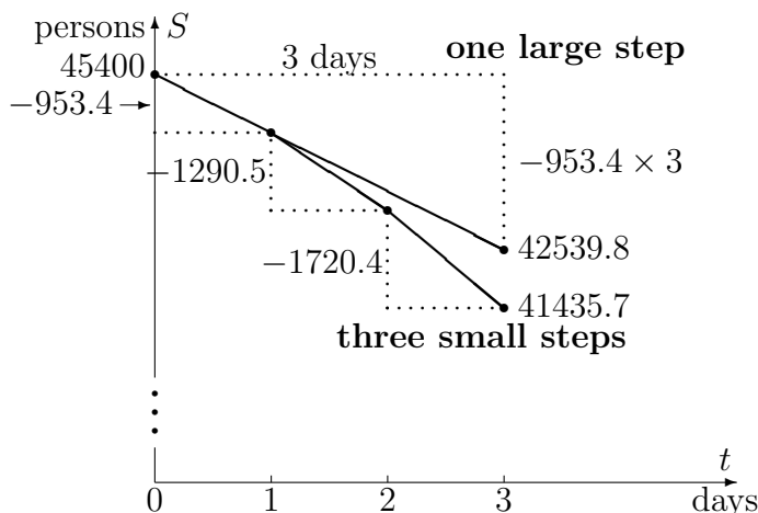
Two approximations to S during the first three days
