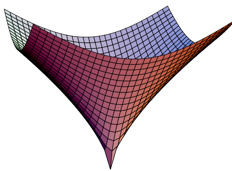
spike: not locally linear
