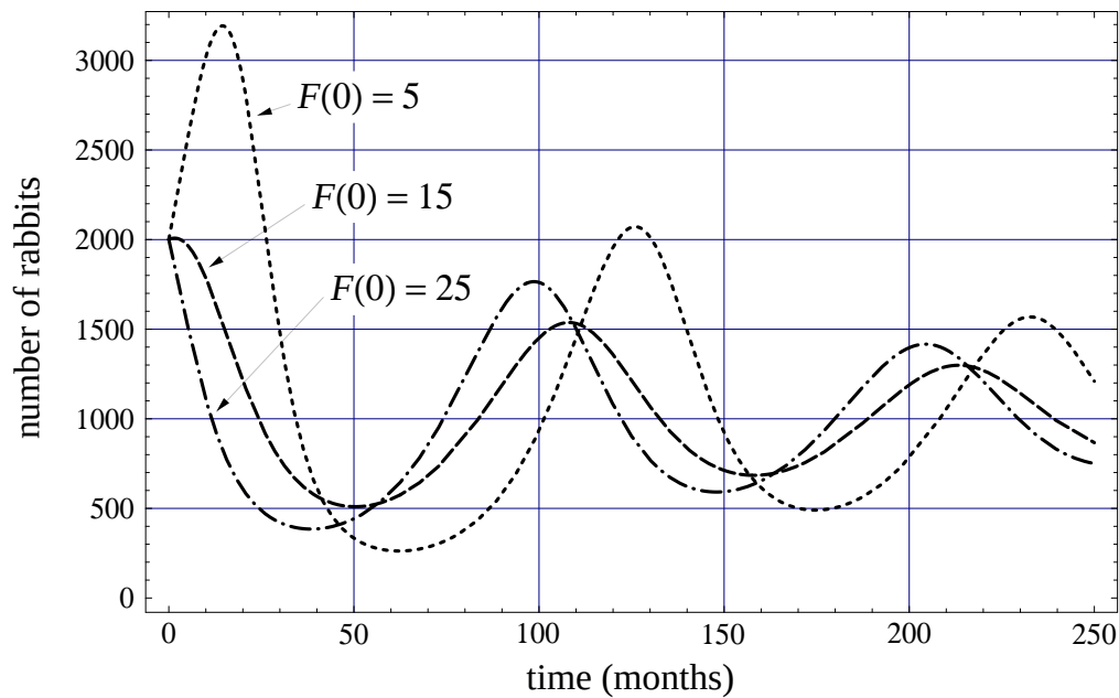
Rabbit populations for different initial fox populations
