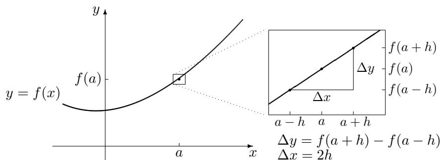
Estimating the value of the derivative f'(a)
