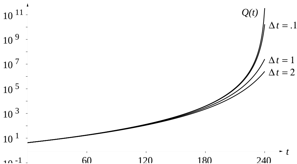
Euler approximations and the formula for Q
