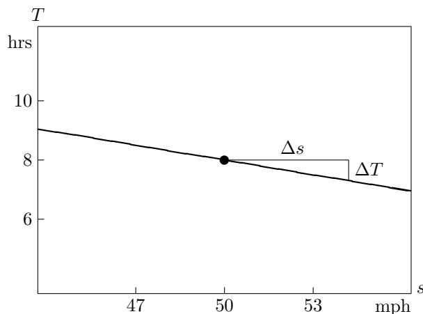
How travel time changes with speed around 50 miles per hour
