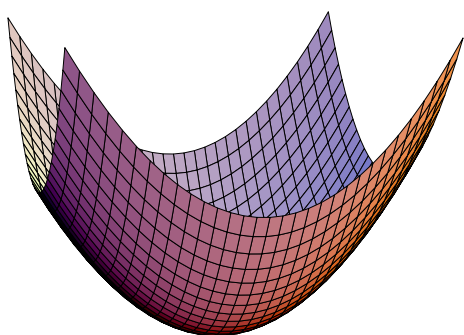
bowl: locally linear
