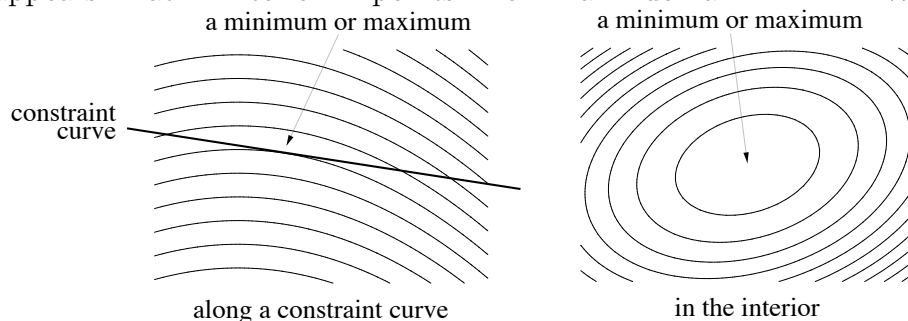
Patterns of contour lines at an extreme point
