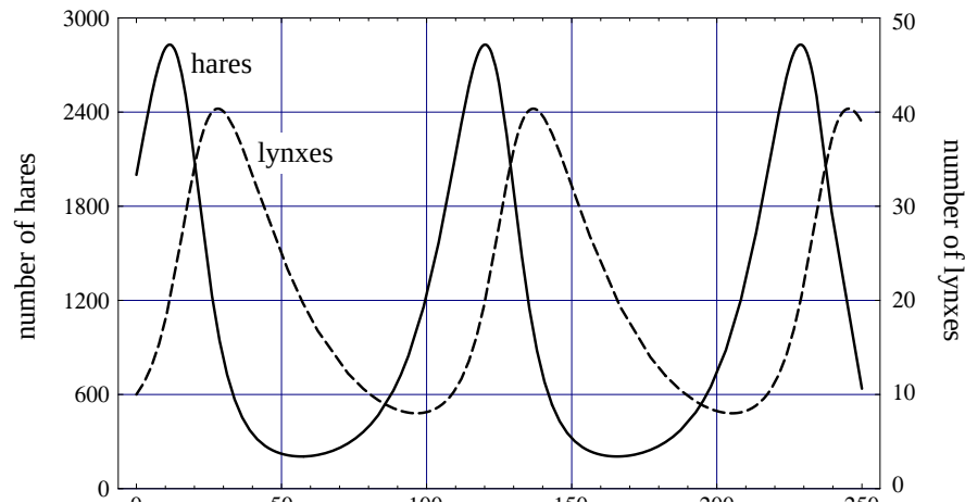
Hare and lynx populations as a function of time
