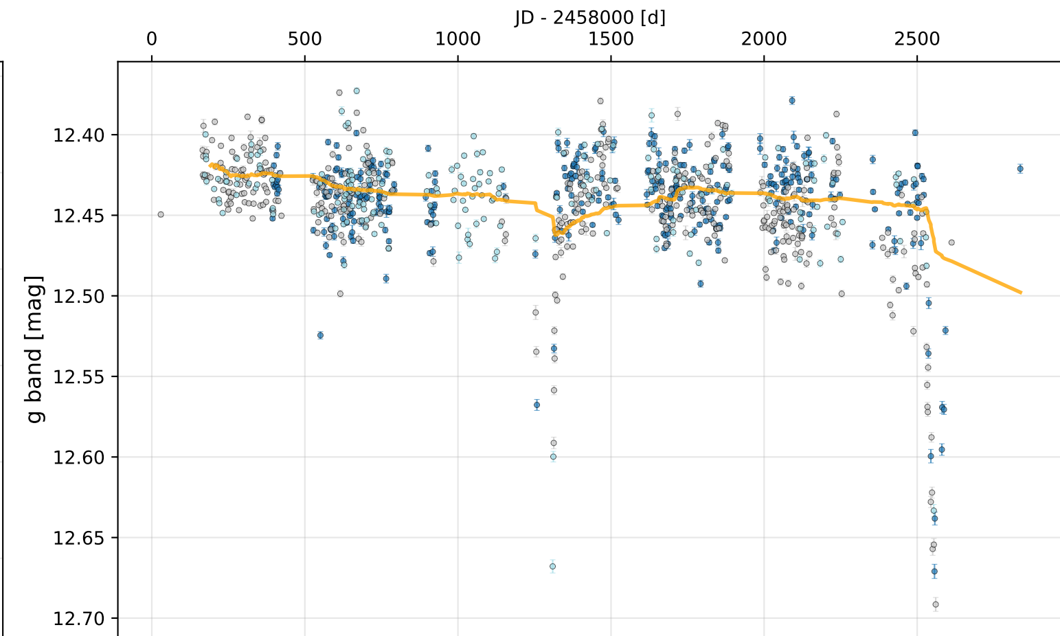
J181752-580749 (644245387906) - Multiple Eclipse Binaries - SkyPatrol LC - JD 2456778-2460837
