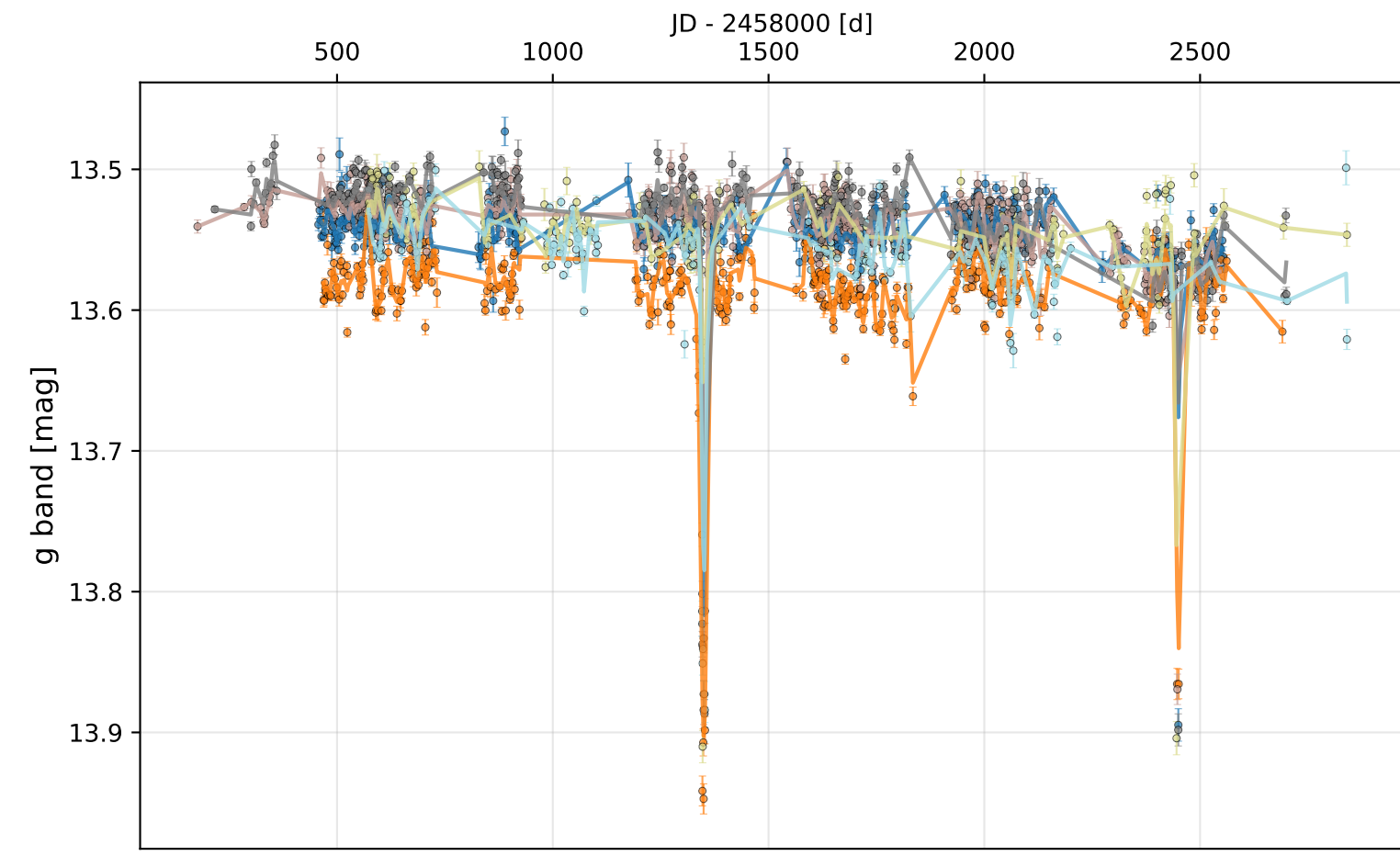
J124745-622756 (515397118400) - Multiple Eclipse Binaries - SkyPatrol LC - JD 2457424-2460840
