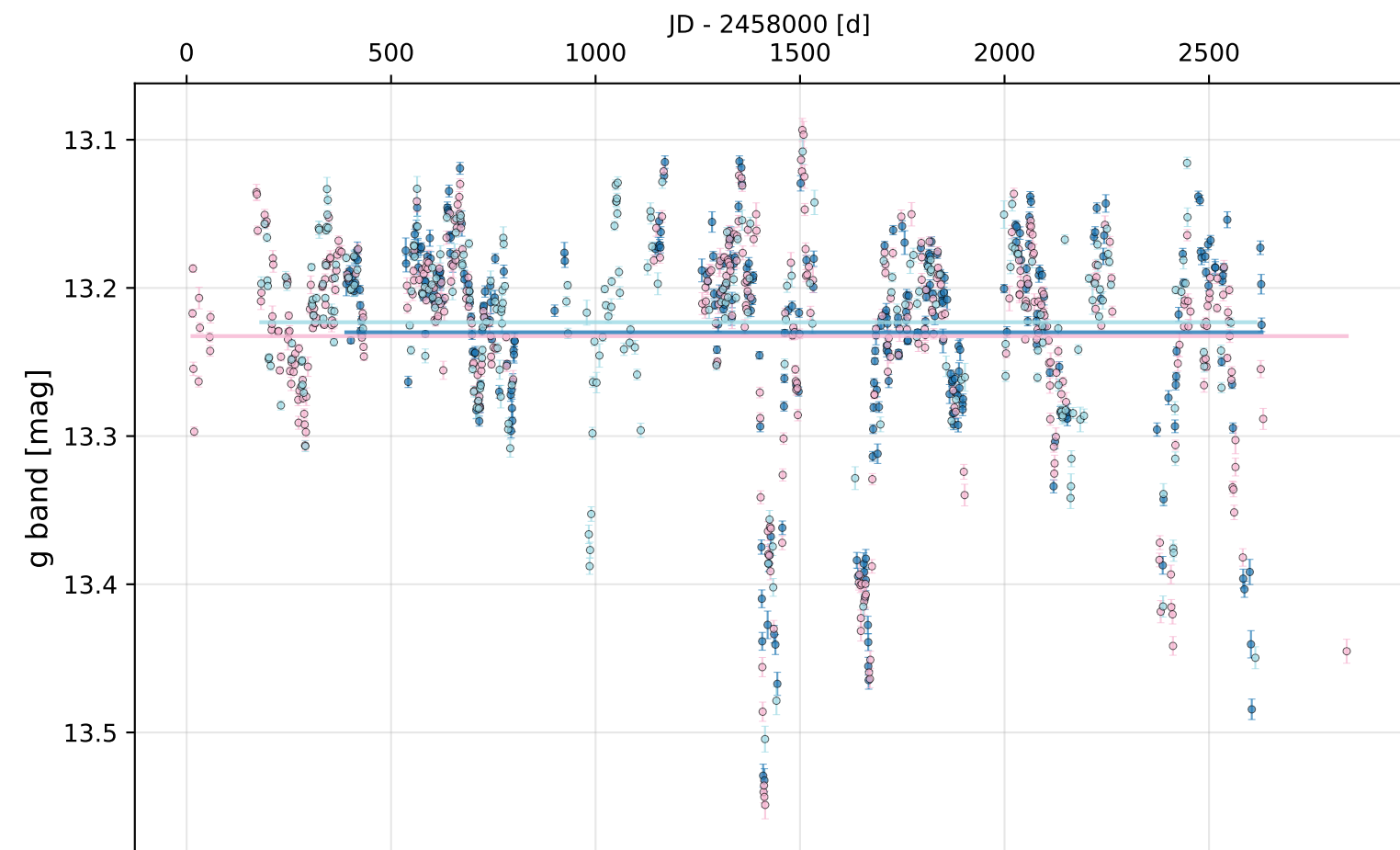
J184916-473251 (472447294641) - Dippers - SkyPatrol LC - JD 2456778-2460837
