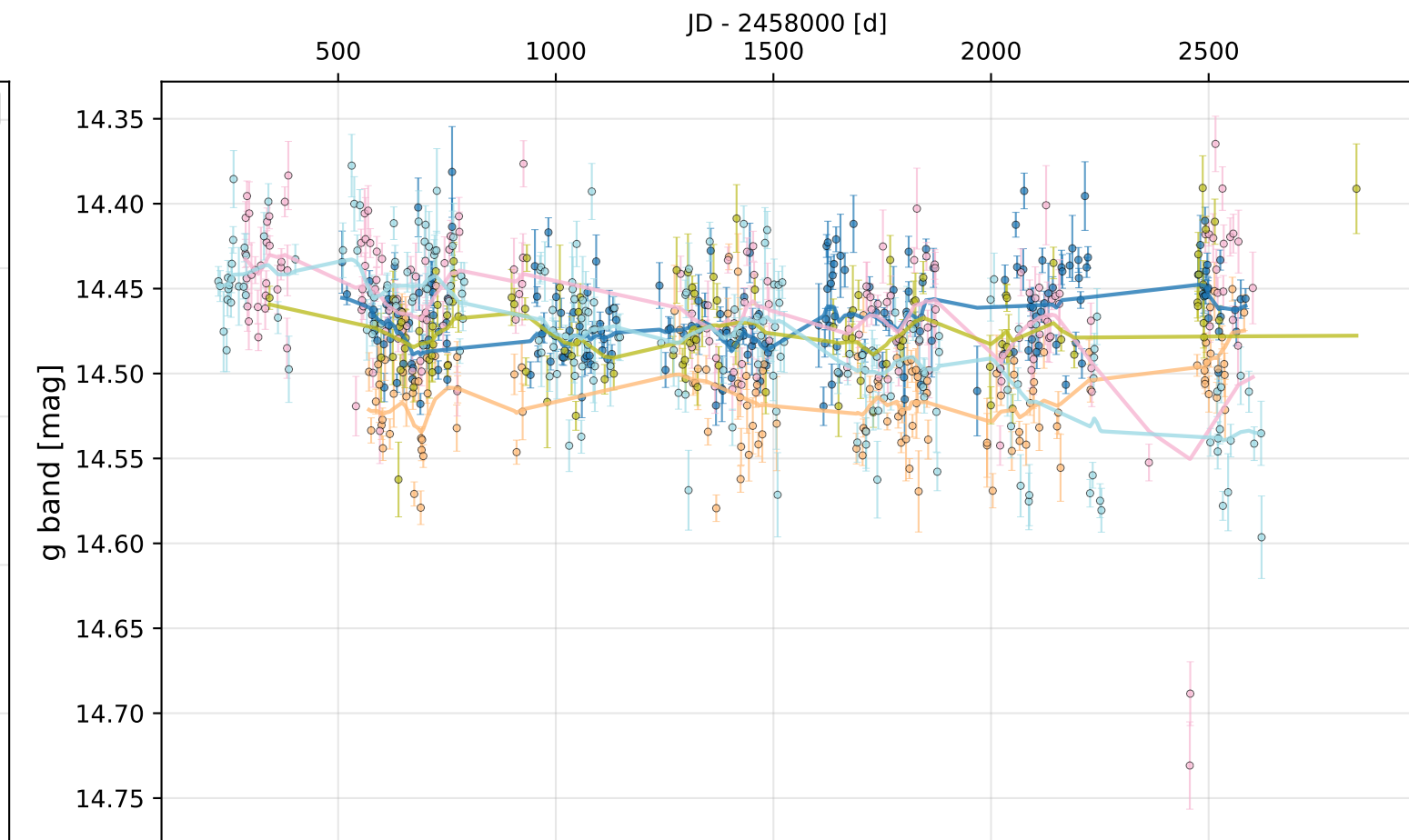
J175602+013135 (231929175915) - Single Eclipse Binaries - SkyPatrol LC - JD 2457043-2460840
