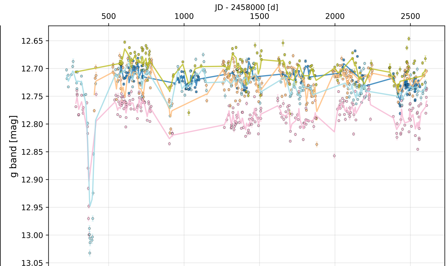
J183210-173432 (317827964025) - Single Eclipse Binaries - SkyPatrol LC - JD 2457078-2460608
