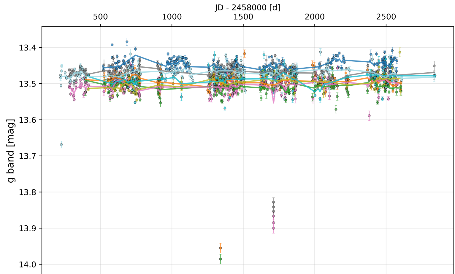
J175912-120956 (326417831663) - Multiple Eclipse Binaries - SkyPatrol LC - JD 2457049-2460842
