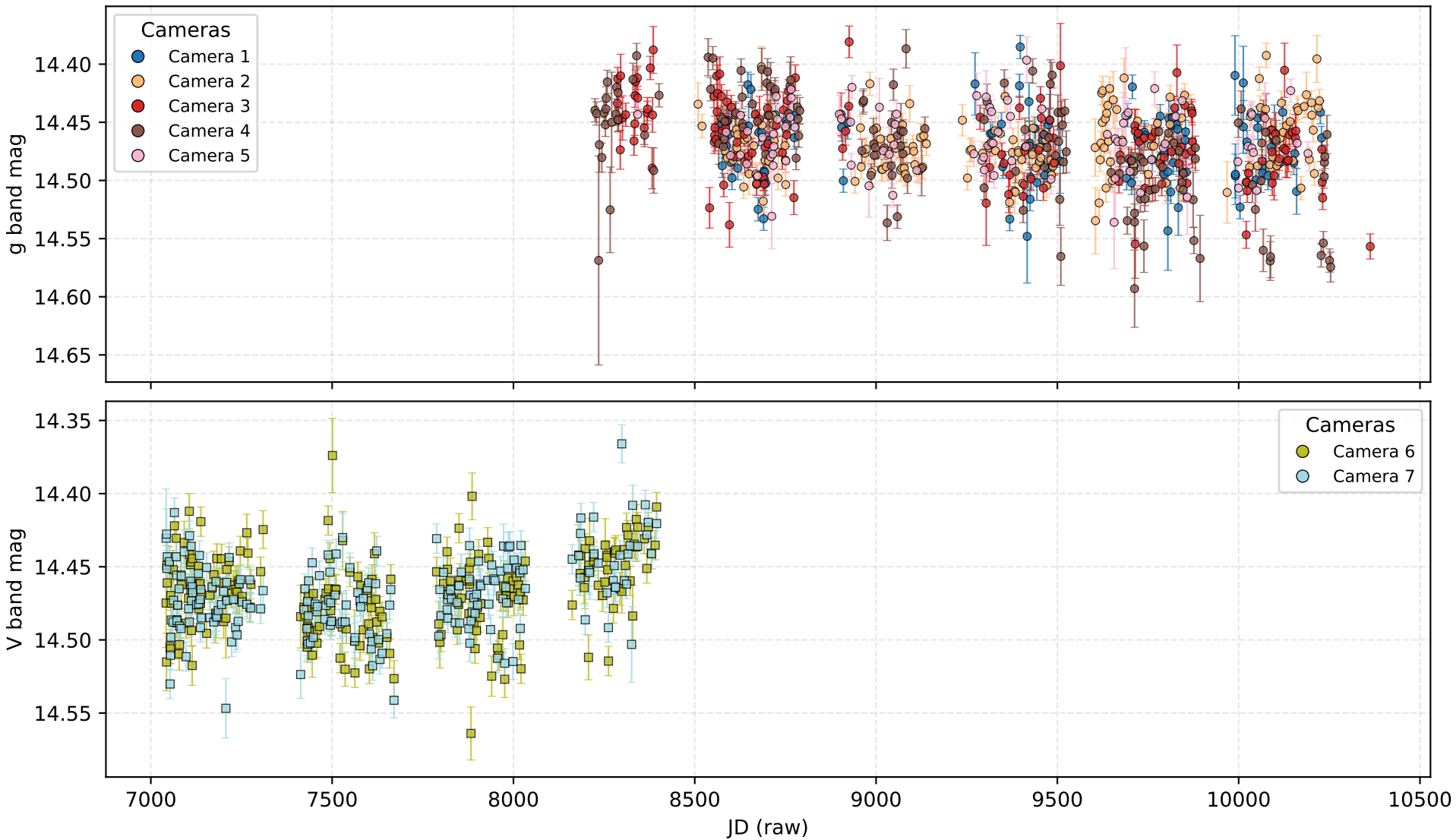
231929175915 - JD 7042-10363 light curve
