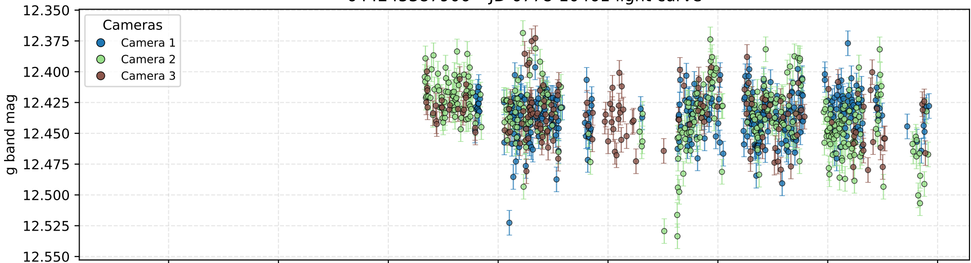
644245387906 - JD 6778-10461 light curve
