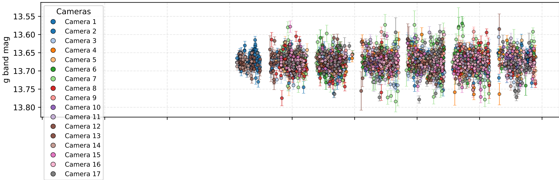
377958261591 - JD 6677-10449 light curve
