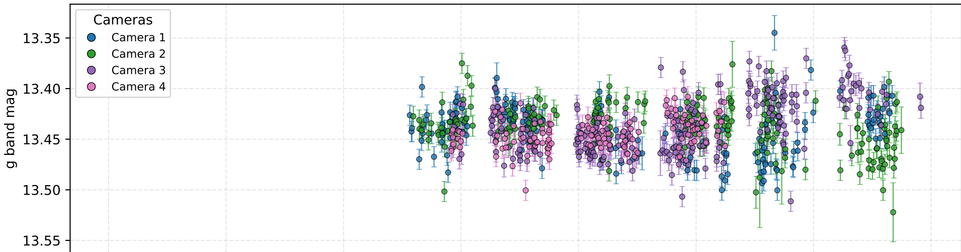
68720274411 - JD 7009-10457 light curve
