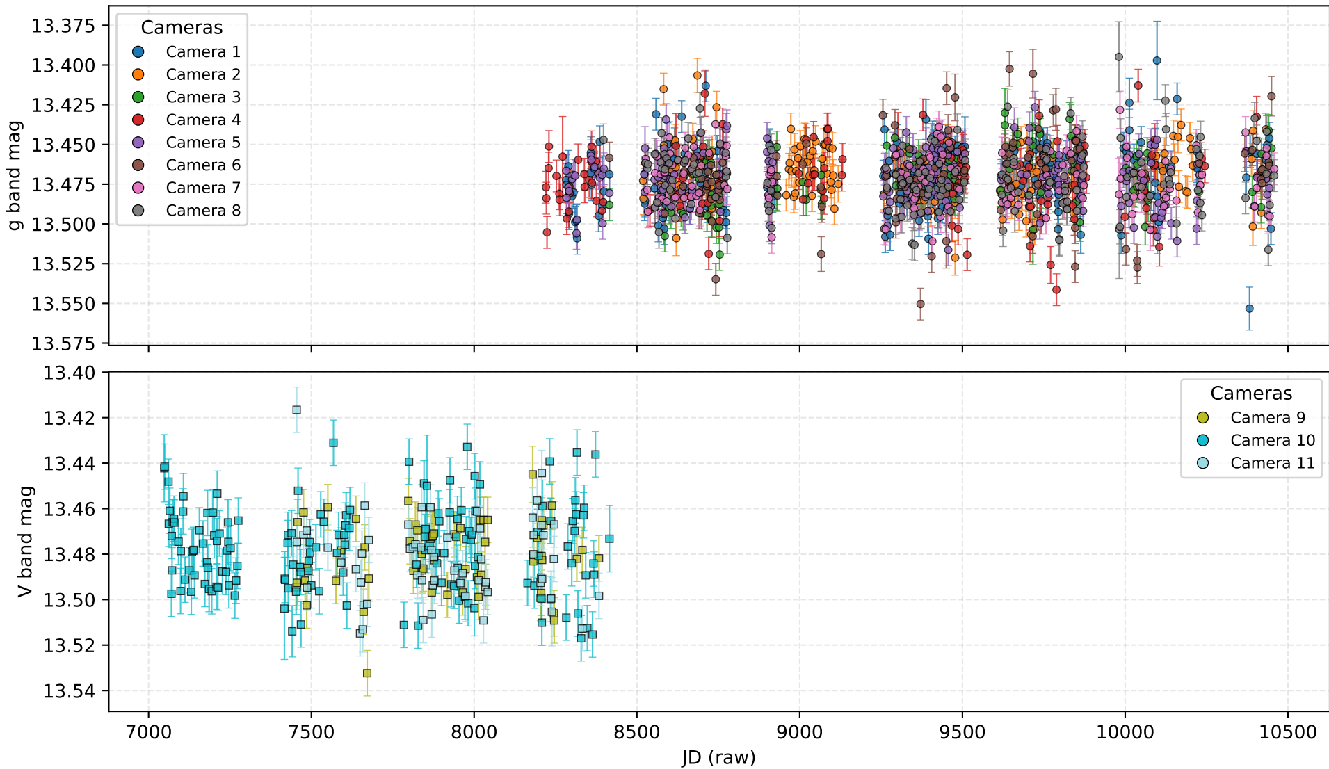
326417831663 - JD 7048-10458 light curve
