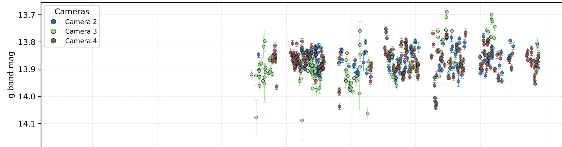
438086901547 - JD 6785-10451 light curve
