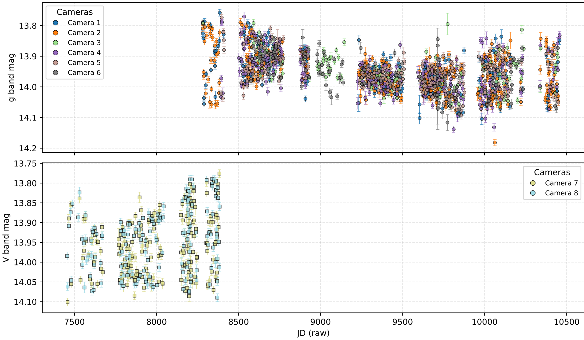
412317159120 - JD 7456-10458 light curve
