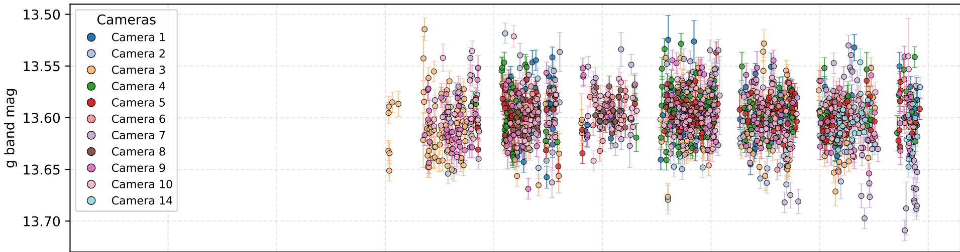
515396514761 - JD 6735-10462 light curve
