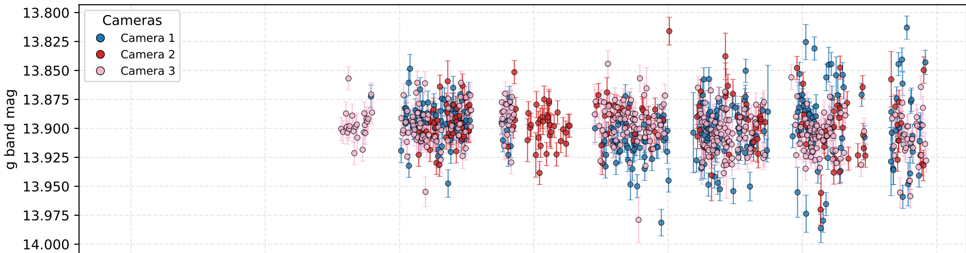
661425129485 - JD 7457-10461 light curve
