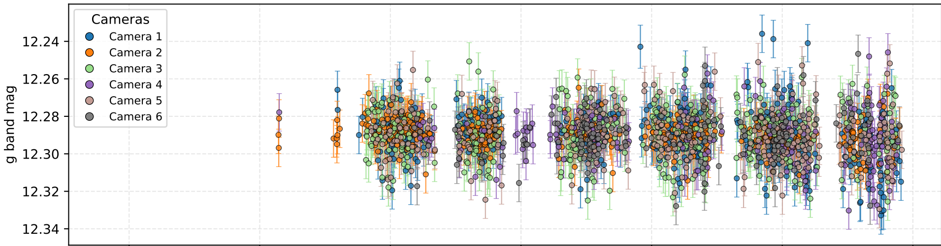
352187470767 - JD 7421-10458 light curve
