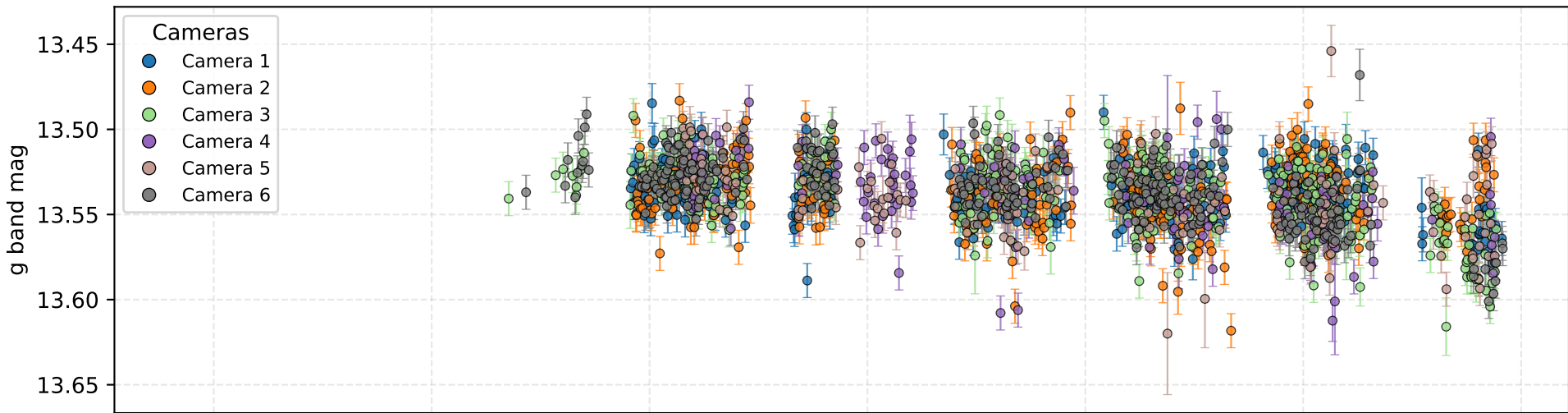
515397118400 - JD 7424-10458 light curve
