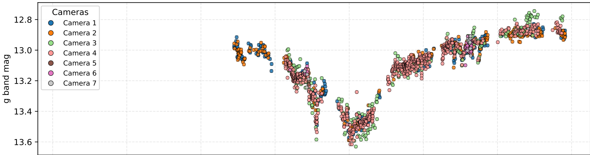
42950993887 - JD 7069-10457 light curve
