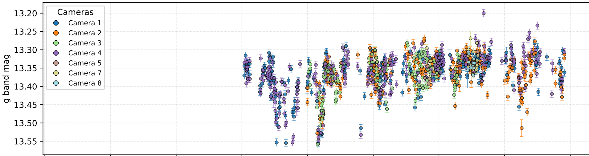
223339338105 - JD 6675-10456 light curve
