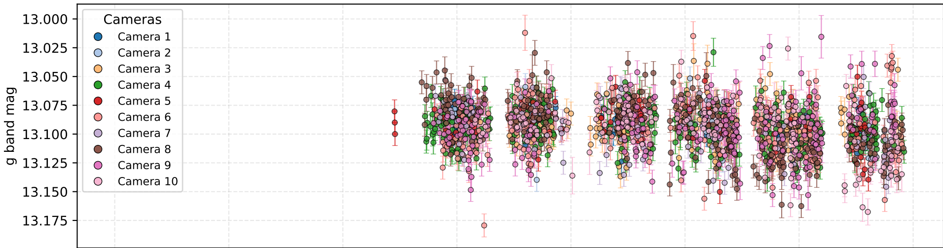
360777377116 - JD 7008-10460 light curve
