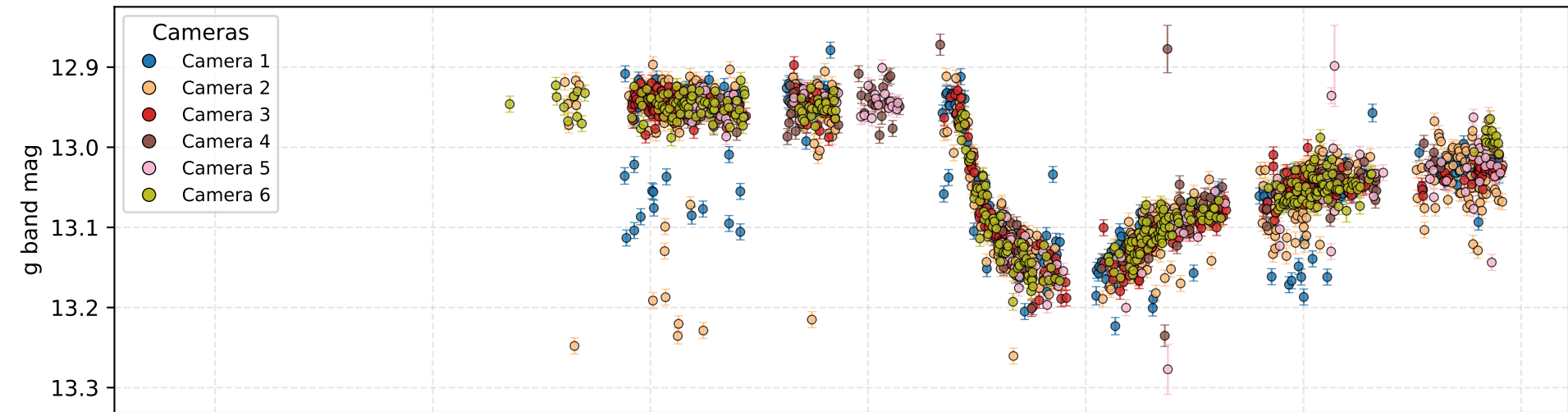
609886184506 - JD 7421-10458 light curve
