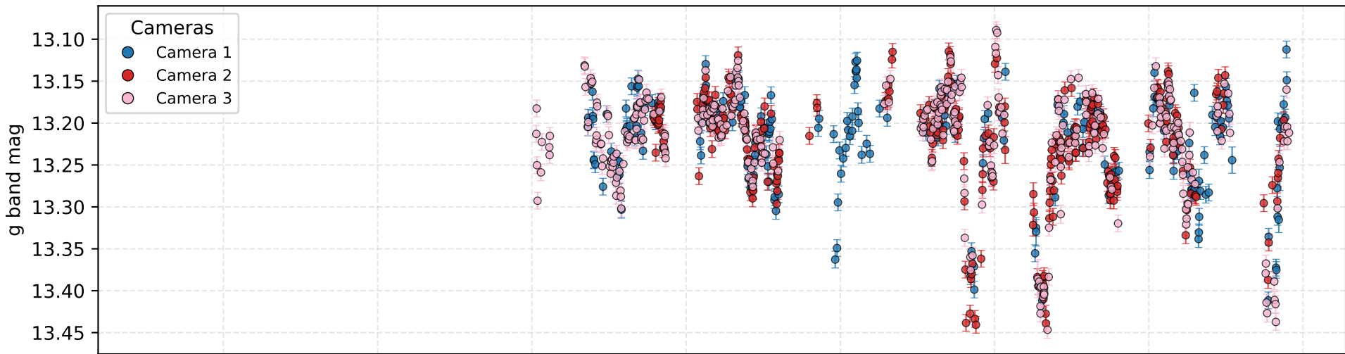
472447294641 - JD 6778-10455 light curve
