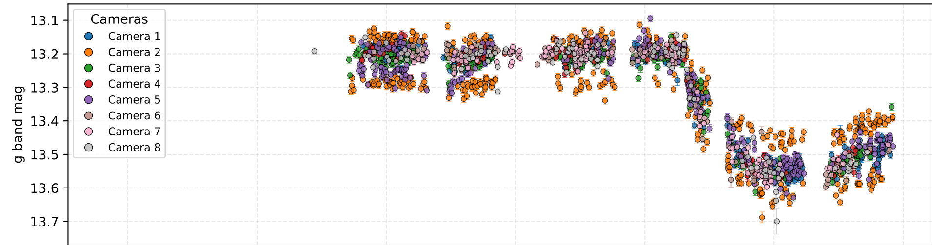
601296043597 - JD 7421-10461 light curve
