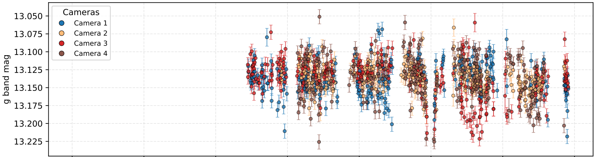
120259184943 - JD 7008-10457 light curve
