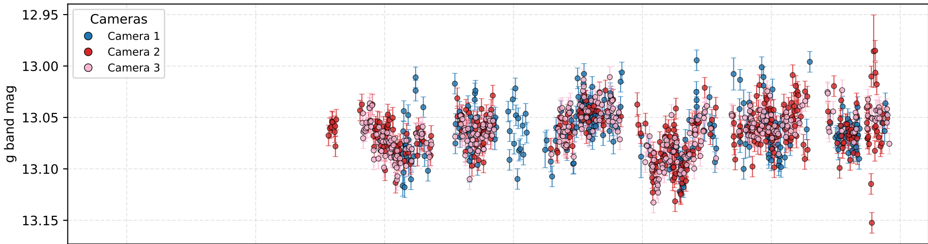
635655234580 - JD 7423-10458 light curve
