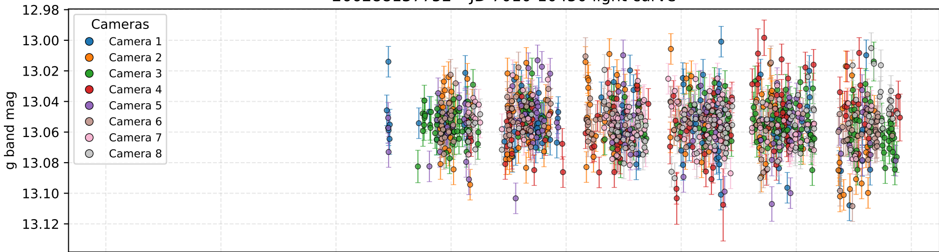
266288137752 - JD 7010-10450 light curve
