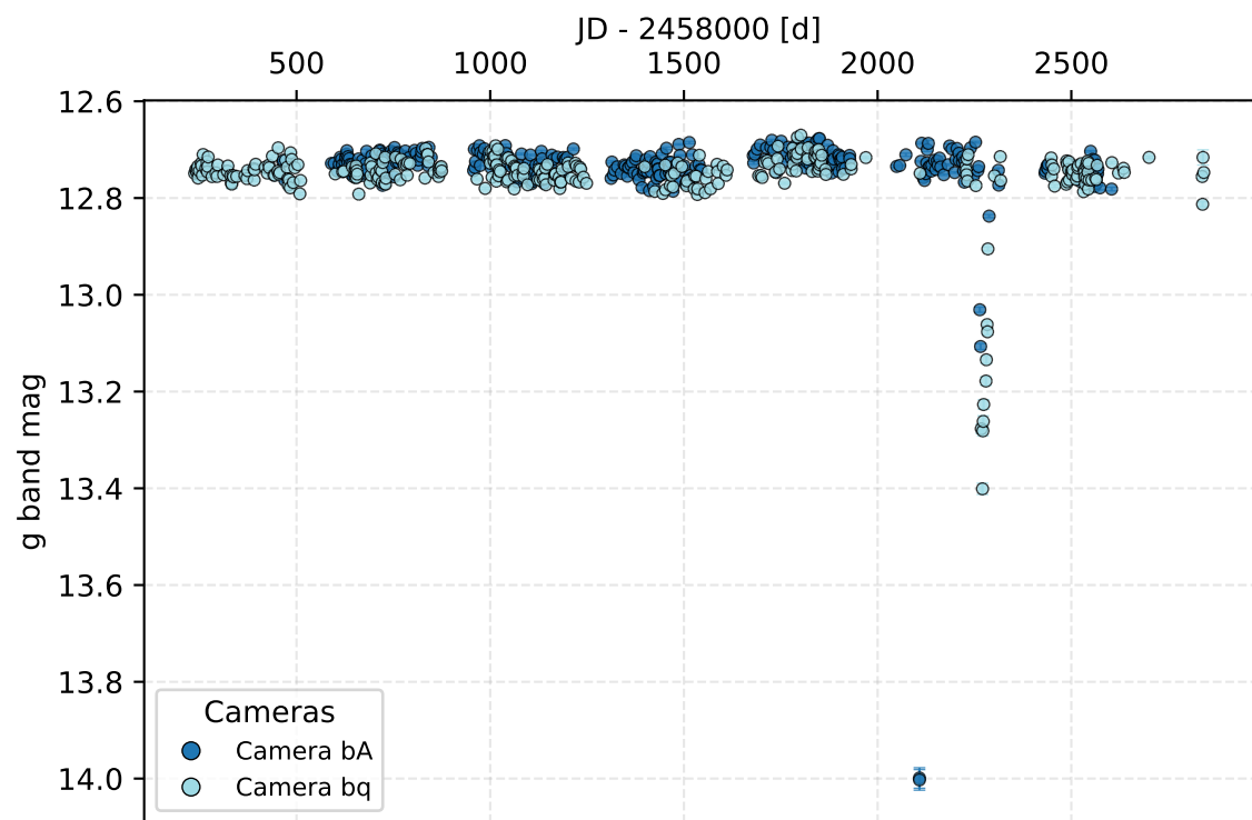
J223332+565552 (60130040391) - Single Eclipse Binaries - JD 2457008-2460842
