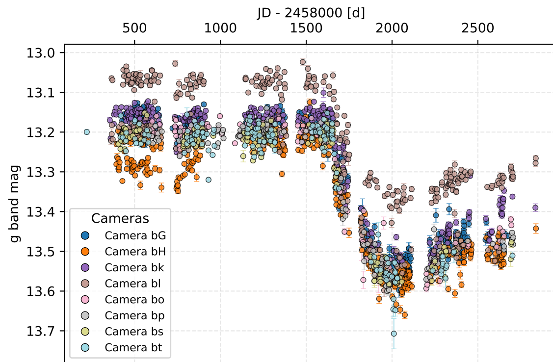
J080327-261620 (601296043597) - Dippers - SkyPatrol LC - JD 2457421-2460838
