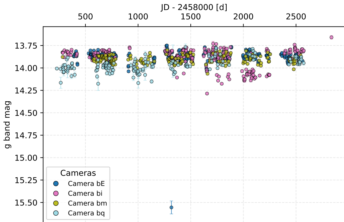
J183606-314826 (438086901547) - Single Eclipse Binaries - SkyPatrol LC - JD 2456785-2460837
