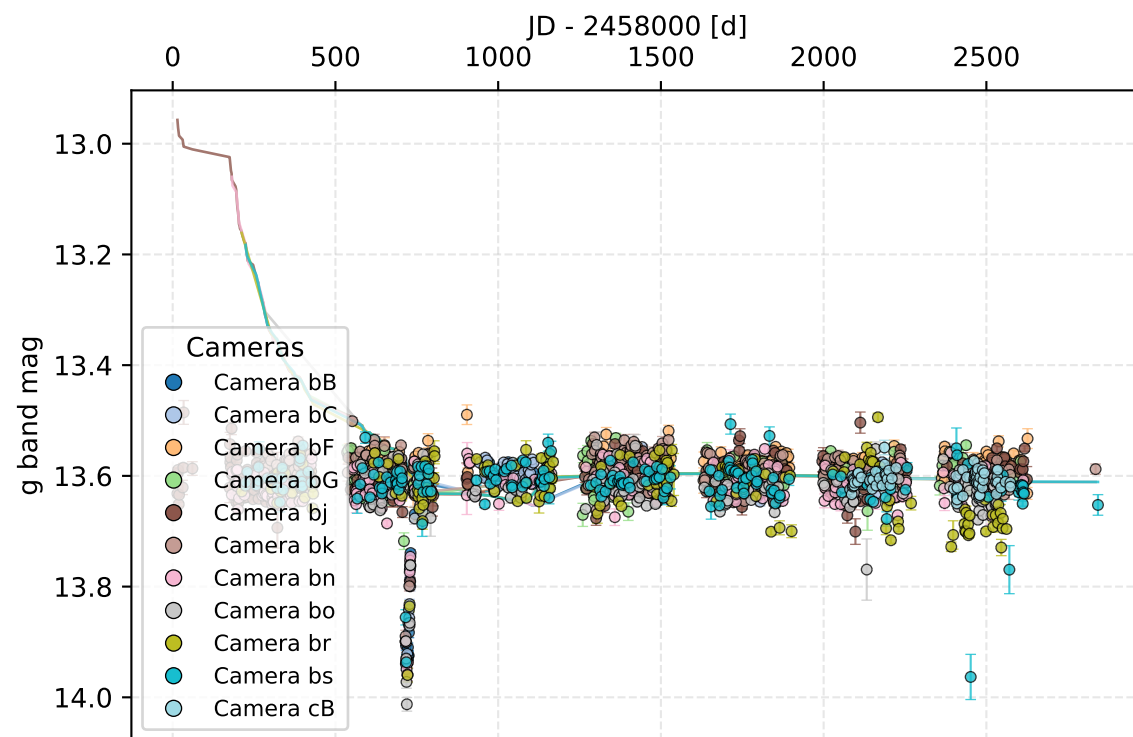
J190316-195739 (515396514761) - Single Eclipse Binaries - SkyPatrol LC - JD 2456731-2460843
