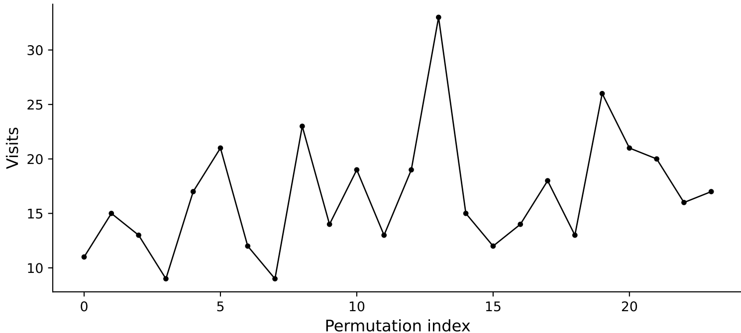
Random walk on S_4 after 400 steps
