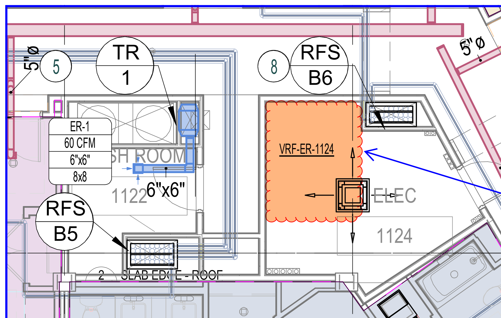
Snap from Mech. drawing M116 LEVEL 11 MECHANICAL PLAN
