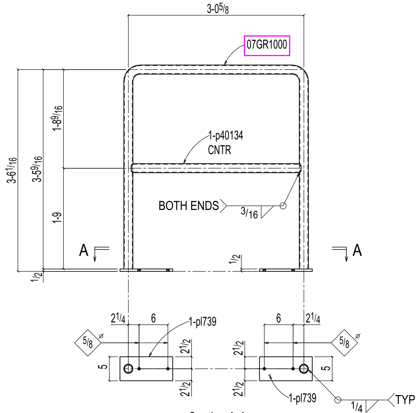
Section A-A 07GR1000 ONE GUARDRAIL 07GR1000
