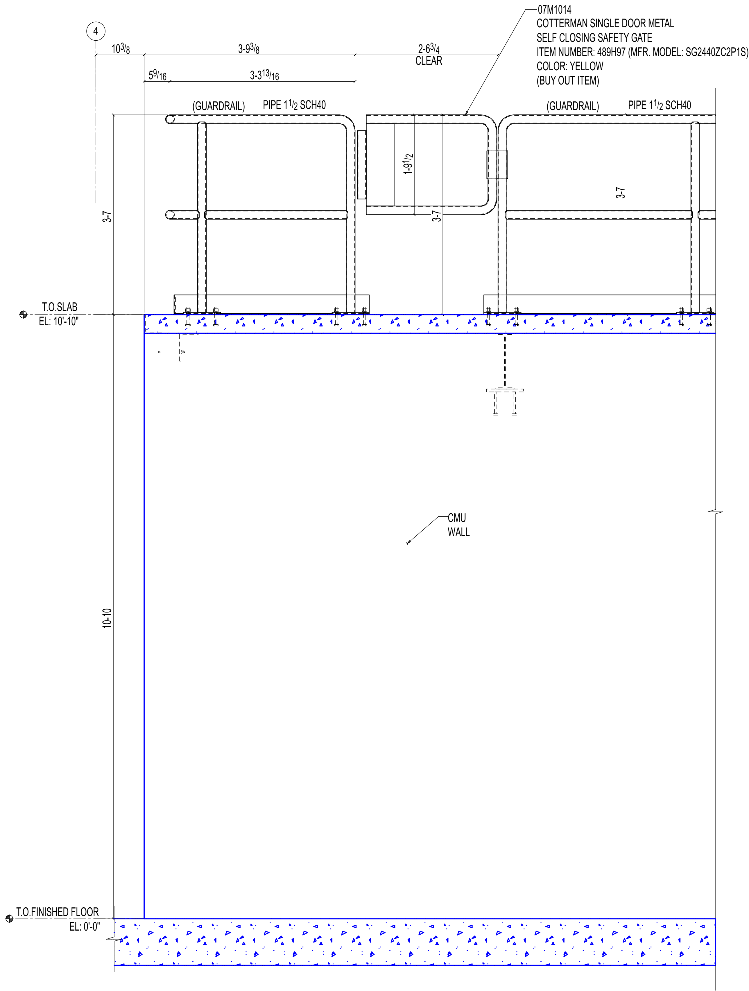
1 ELEVATION SE713 OTHERS NOT SHOWN FOR CLARITY
