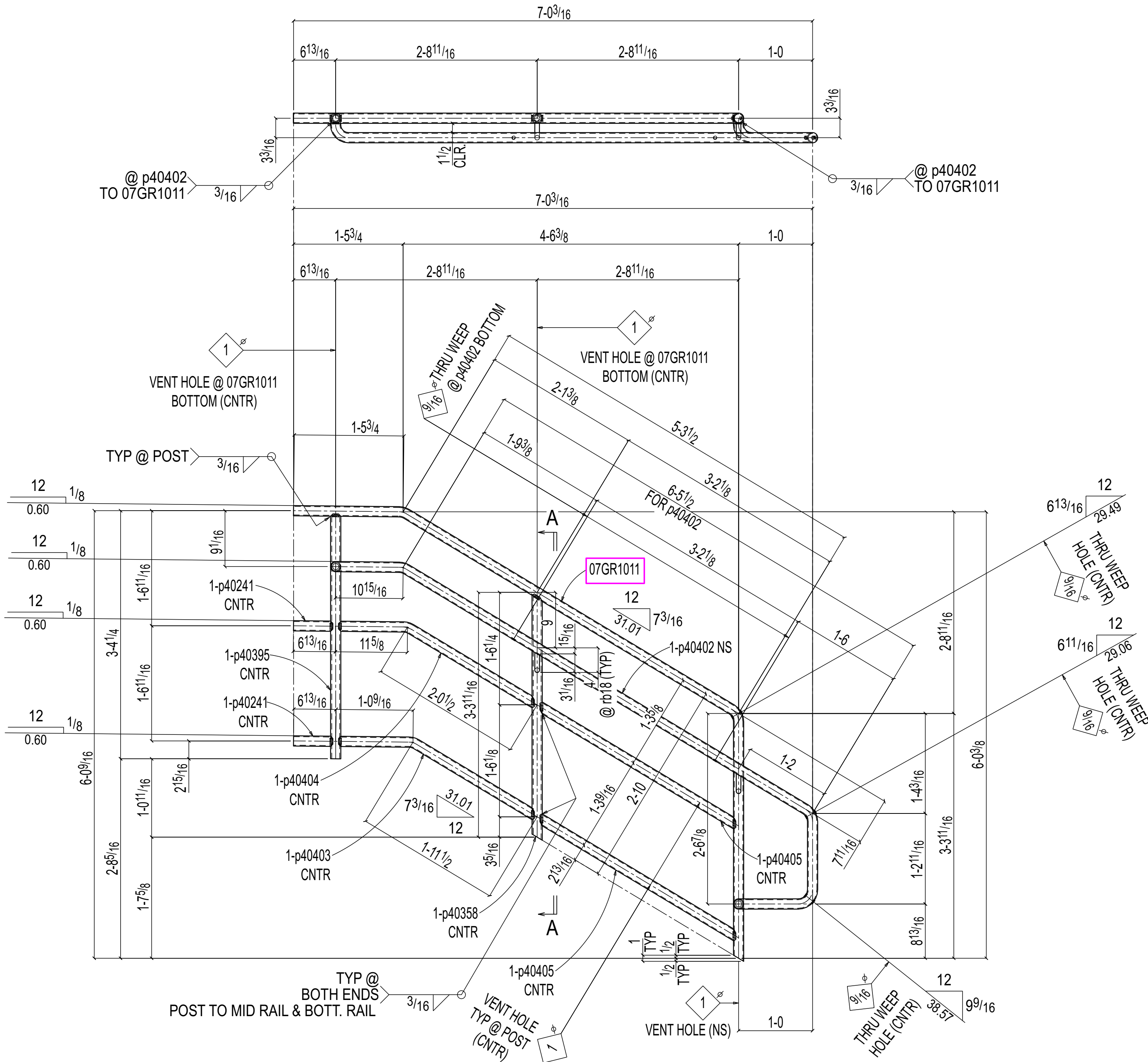
ONE GUARDRAIL 07GR1011
