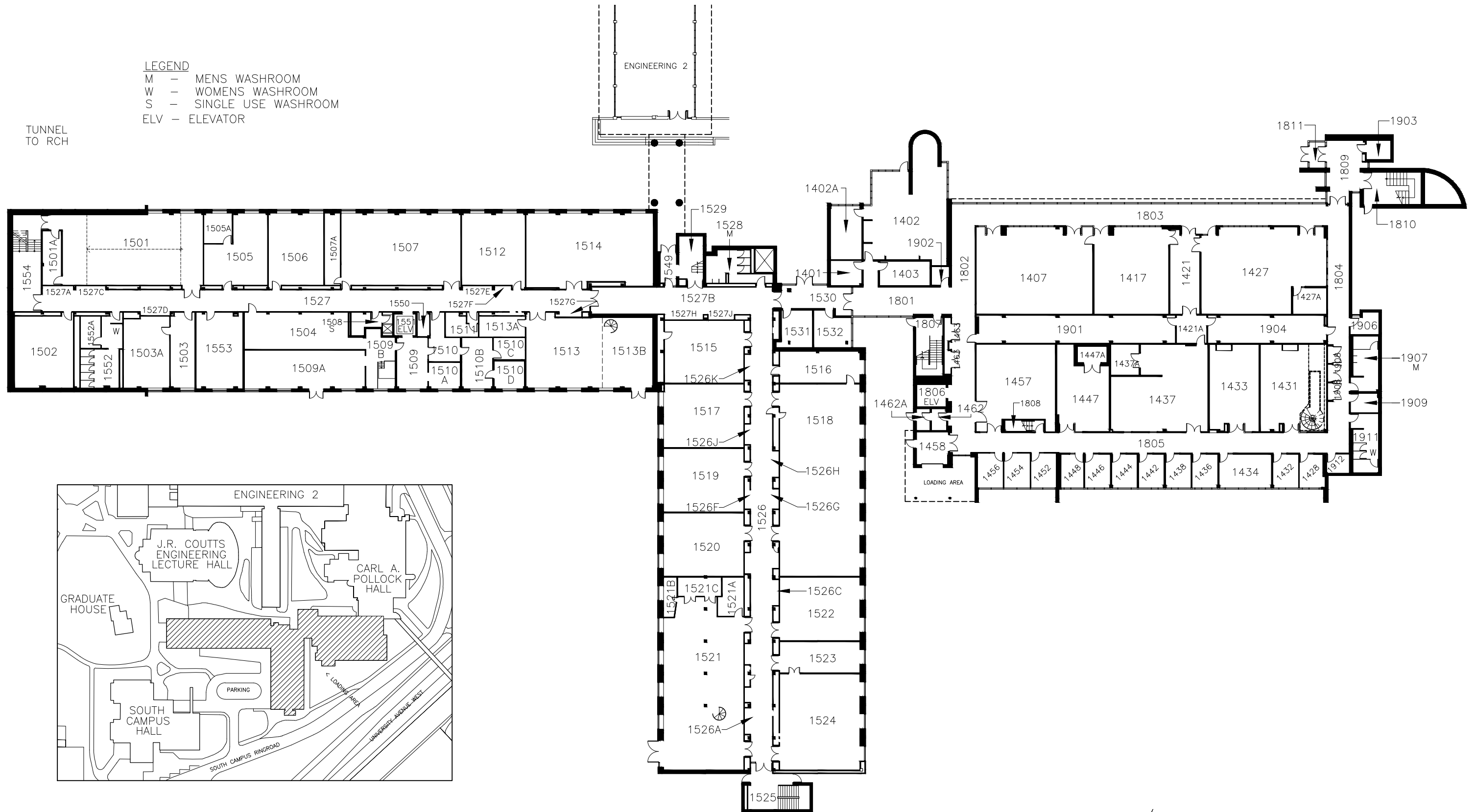
FIRST FLOOR PLAN DOUGLAS WRIGHT ENGINEERING BUILDING No. 01 UNIVERSITY OF WATERLOO UPDATED — MAY 2023
