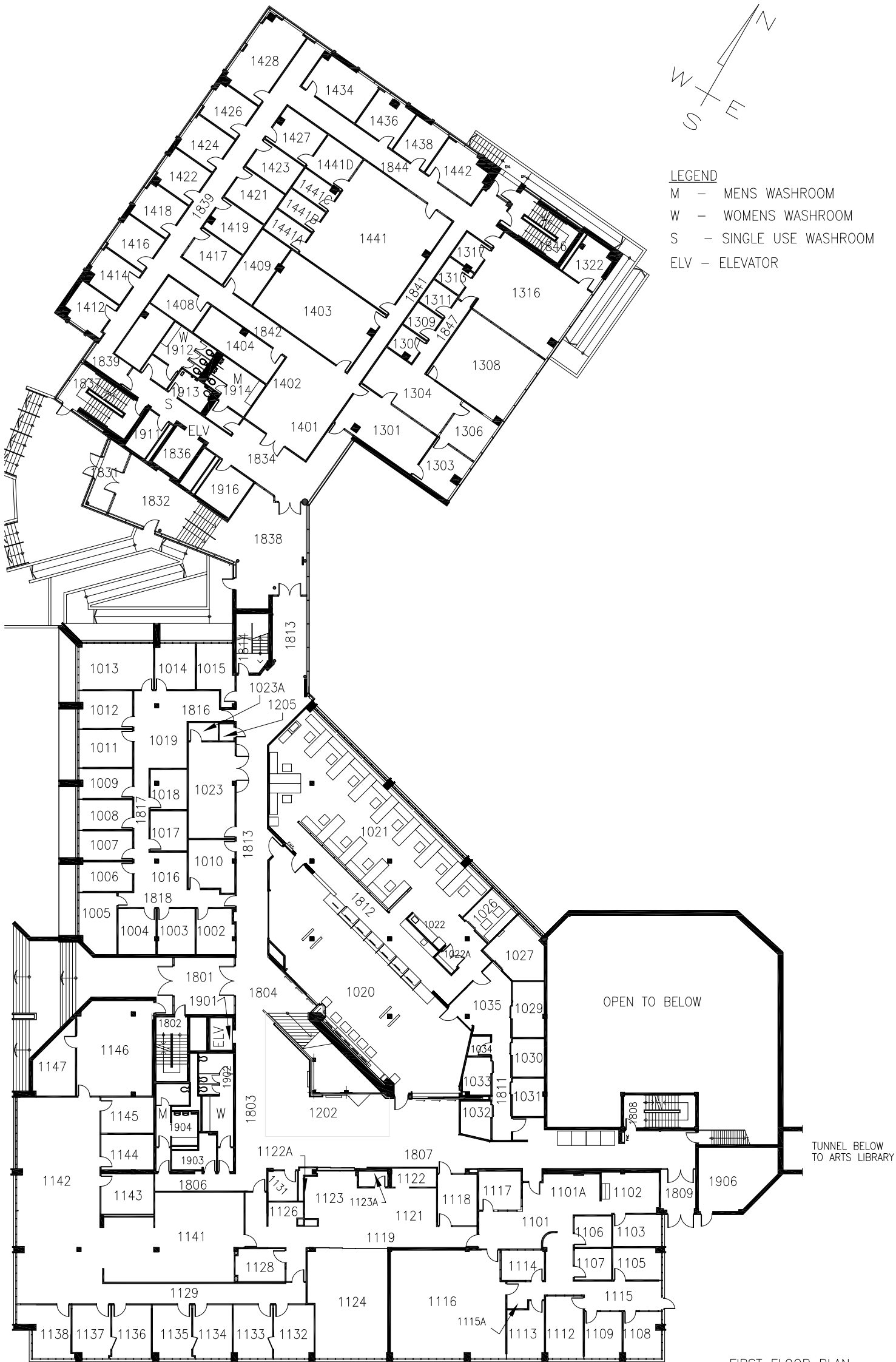
FIRST FLOOR PLAN NEEDLES HALL BUILDING No. 31 UNIVERSITY OF WATERLOO UPDATED – OCT 2023
