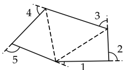
FIGURE 8-22. Pentagon (three triangles).
