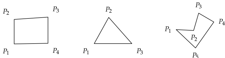
FIGURE 8-19. Simple polygons.
