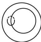
Torus, or doughnut, or anchor ring
