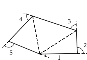
FIGURE 8-22. Pentagon (three triangles).
