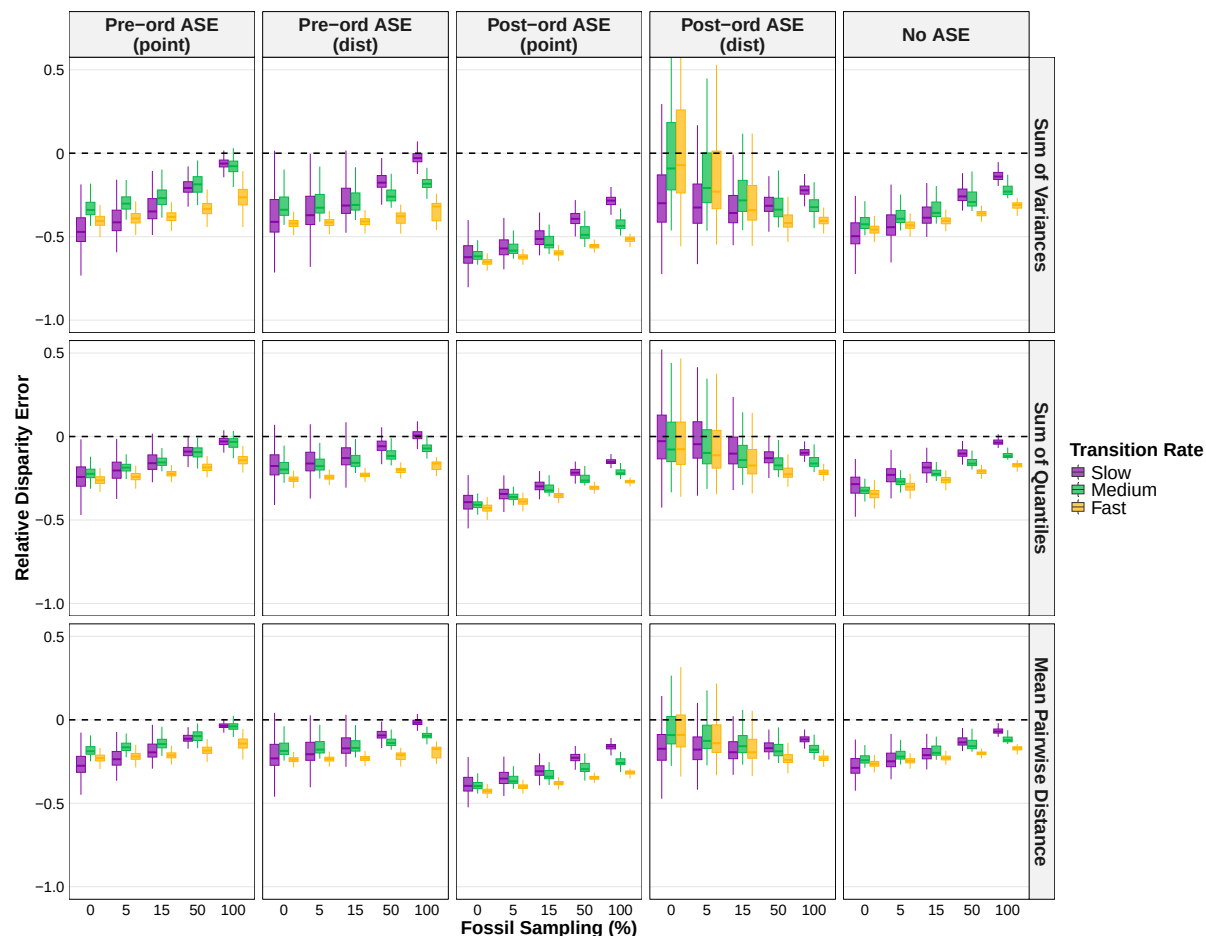
Figure 6: fixed axes Relative disparity error returned from pre-ordination point ASE (ancestral state estimation), pre-ordination distribution ASE, post-ordination point ASE, post-ordination distribution ASE and no ASE. These disparity errors were calculated across three transition rates (fast (0.9), medium (0.1) and slow (0.01)), five simulated fossil sampling densities (100%, 50%, 15%, 5% and 0%) and three disparity metrics (Sum of variances, sum of quantiles and mean pairwise distance). Values closest to 0 (dotted horizontal line) were most accurate; negative errors are under-estimates and positive are over-estimates.
