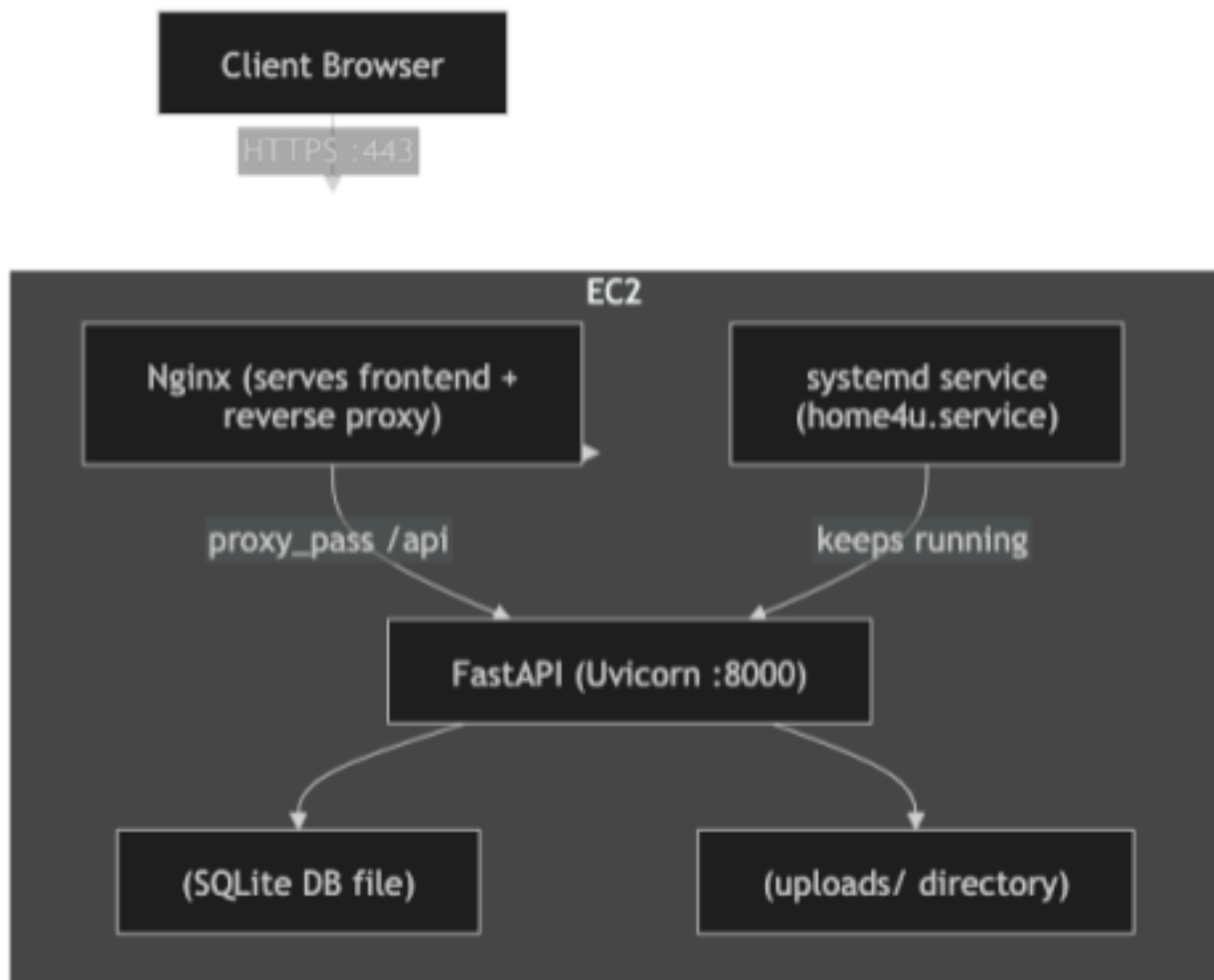
Figure 2 — Home4U Deployment Architecture
