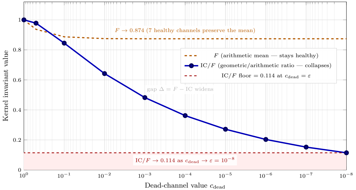
FIG. 4. Geometric slaughter: one dead channel destroys multiplicative coherence while leaving the arithmetic mean nearly intact. An 8-channel trace with 7 channels at c = 0.999 and 1 channel at c_{\text{dead}} . As the dead channel approaches \epsilon = 10^{-8} , IC/F (blue) drops from 1.000 to 0.114, but F (orange) falls only from 0.999 to 0.874—a diverging heterogeneity gap \Delta = F - IC . This mechanism underlies confinement detection [25] in the Standard Model closure [3]: the color channel at c \approx \epsilon in hadrons produces IC/F < 0.04 , making the quark→hadron boundary visible as a 100× drop that F alone would miss.
