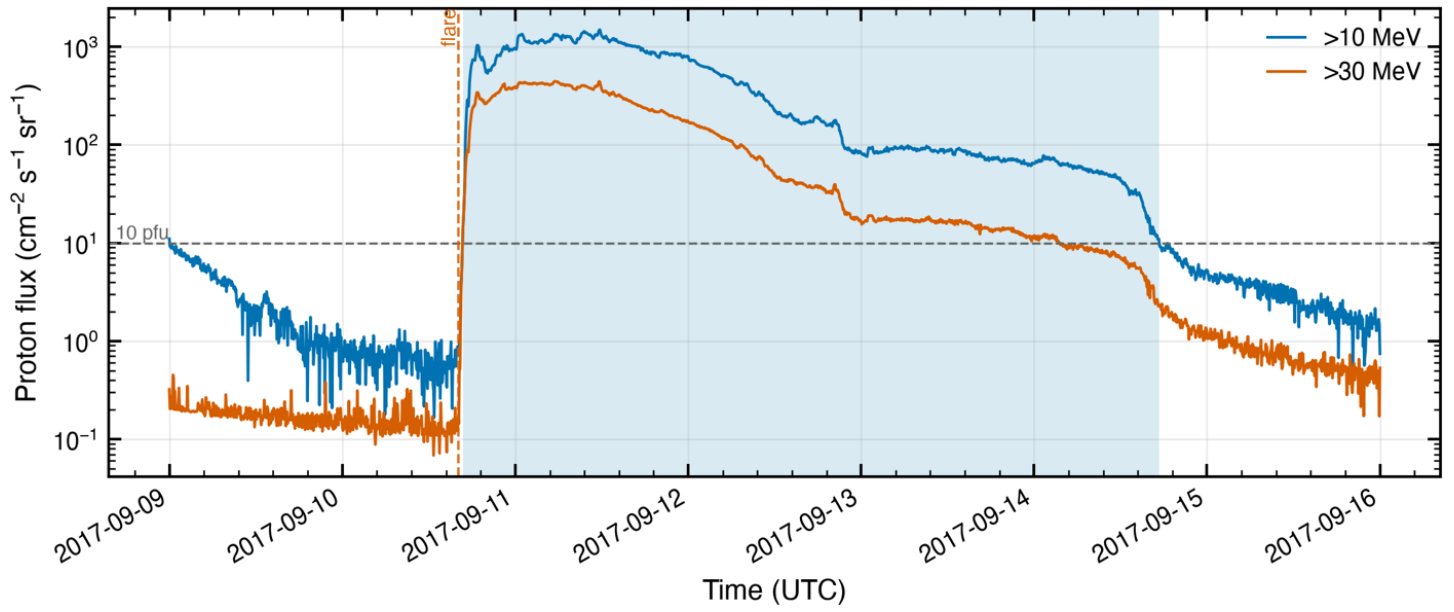
SEP event detection — S3 radiation storm
