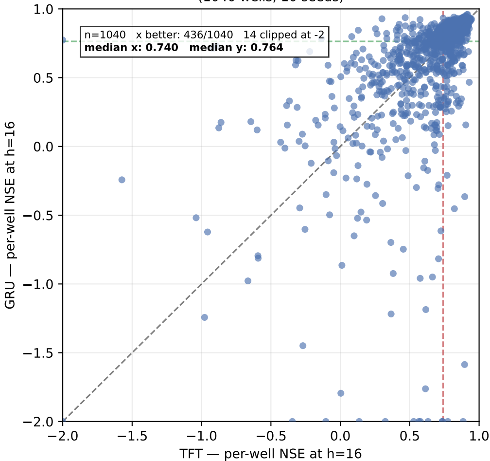
GRU vs TFT: per-well NSE at h=16 (1040 wells, 10 seeds)
