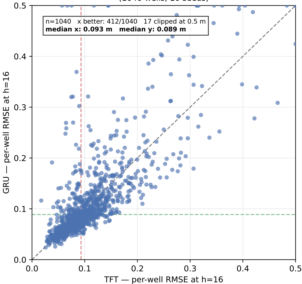
GRU vs TFT: per-well RMSE at h=16 (1040 wells, 10 seeds)
