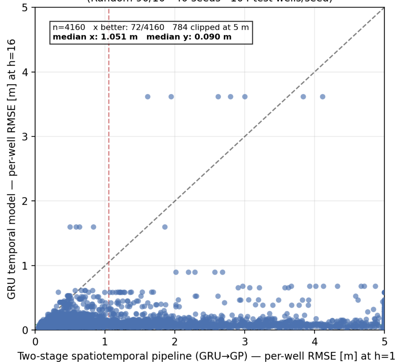
Two-stage spatiotemporal pipeline vs GRU direct forecast (Random 90/10 · 40 seeds · 104 test wells/seed)
