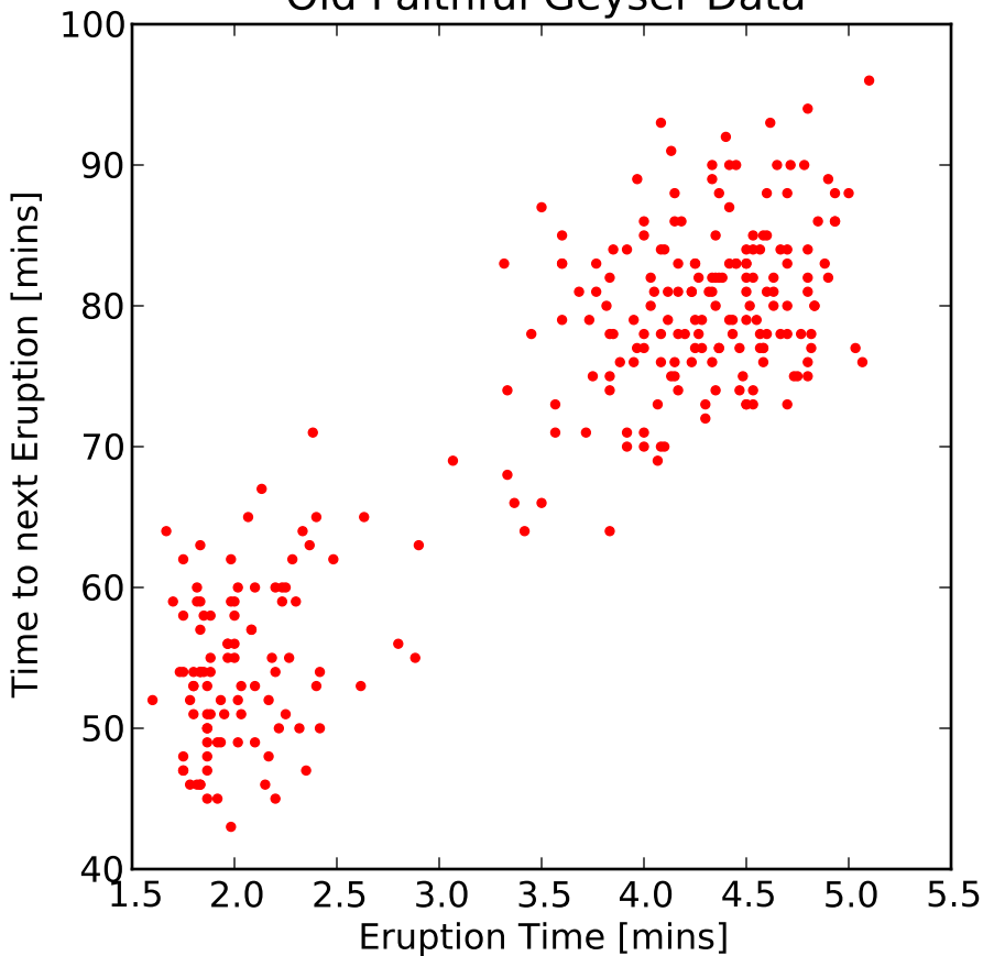
Old Faithful Geyser Data
