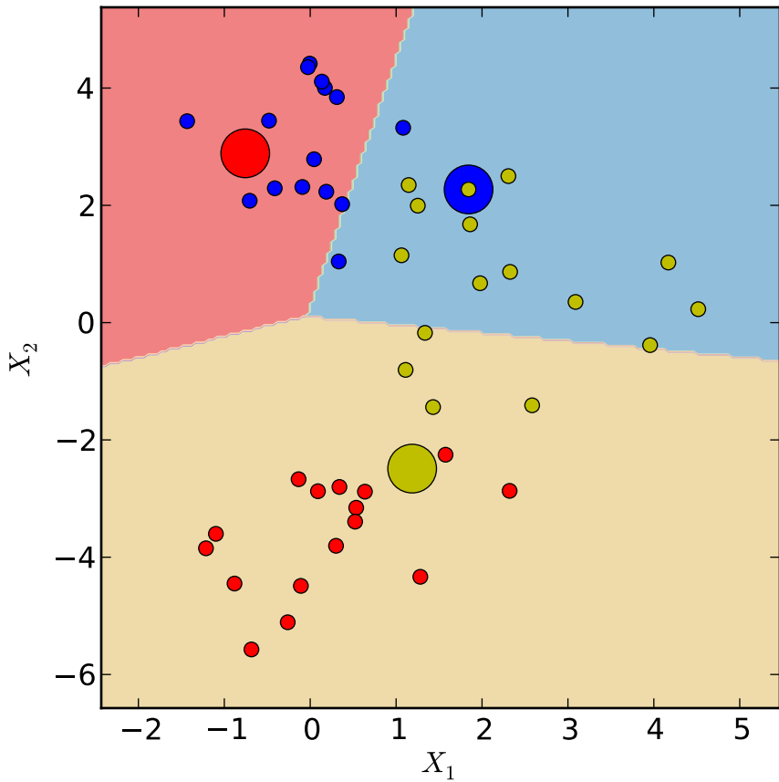
Iteration 5
