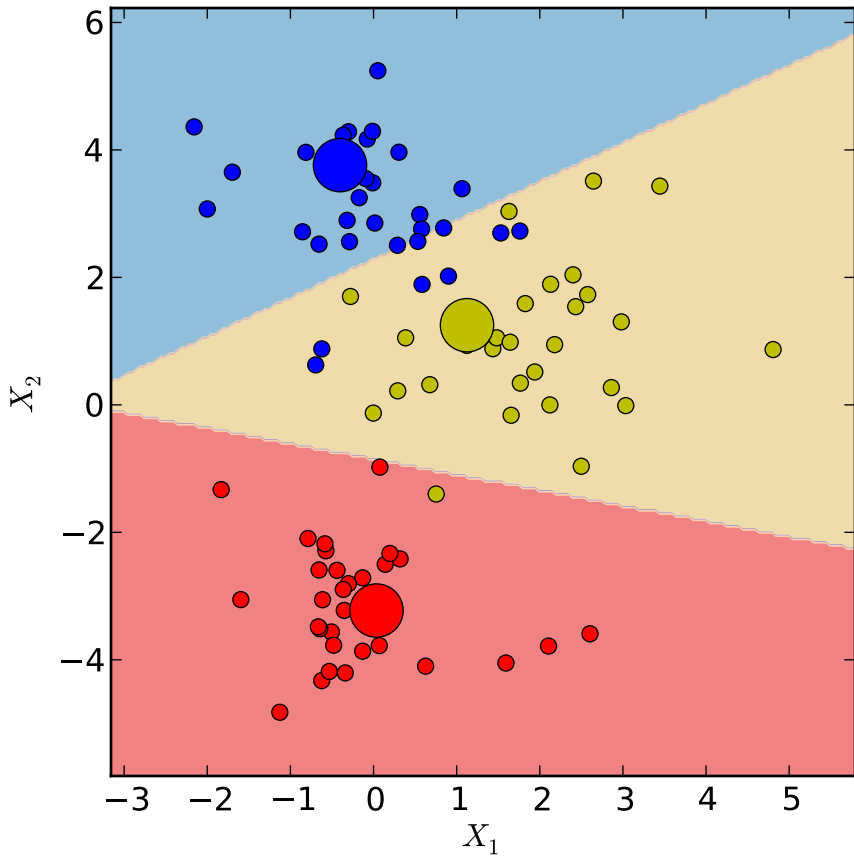
Online K-means
